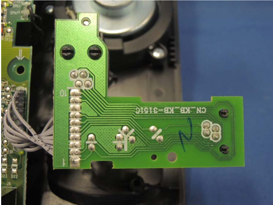
Deskset AC Jack and Telephone Line Jack rear side
