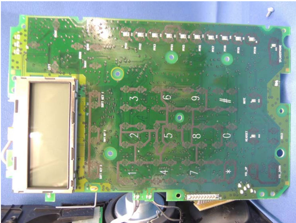
Deskset Main PCB solder side (View 1)
