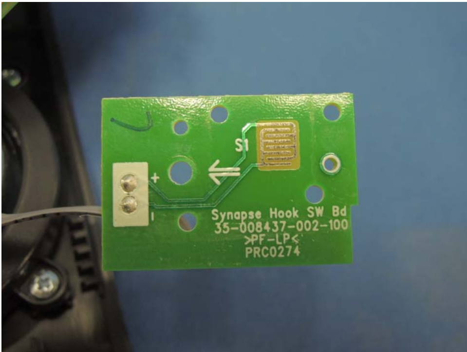
Deskset Hook Switch Board front side
