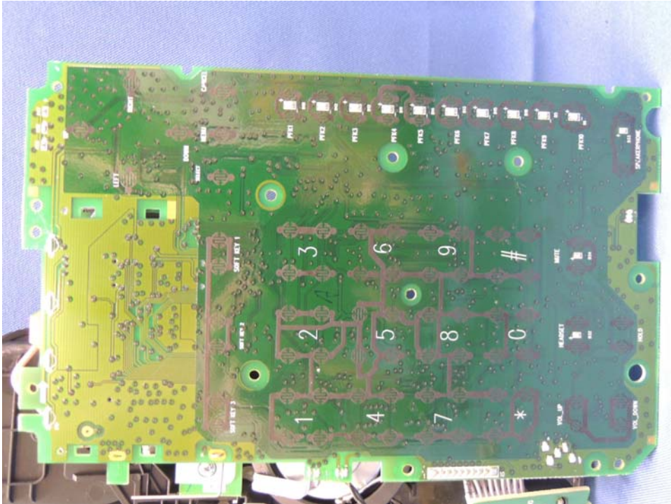
Deskset Main PCB solder side (View 2)
