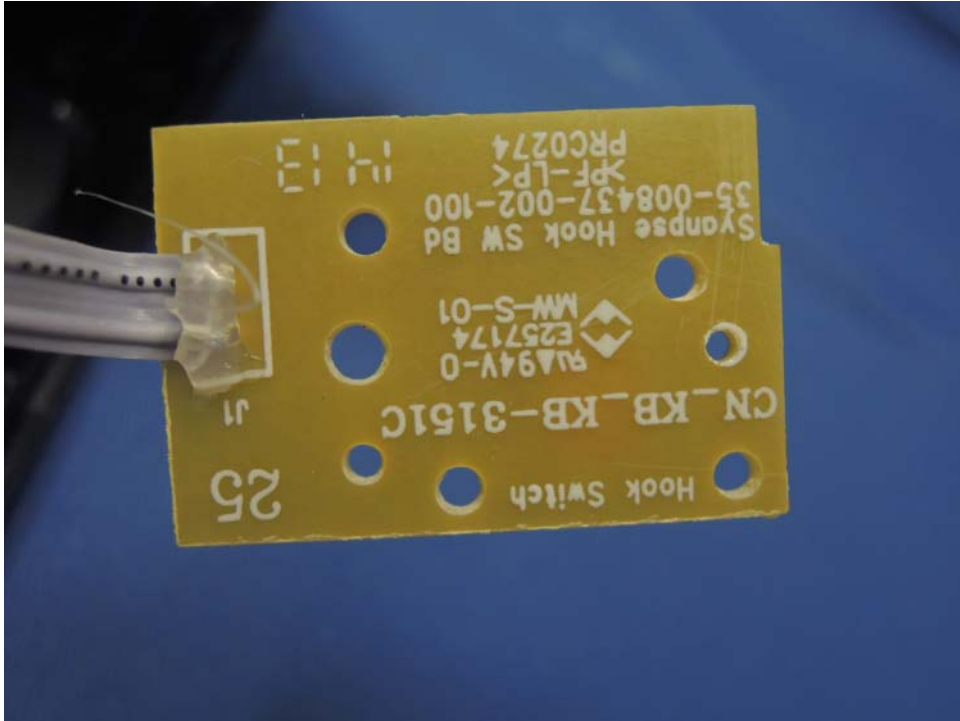
Deskset Hook Switch Board rear side
