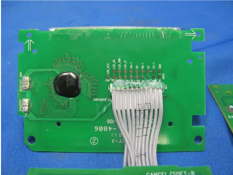
Base Unit LCD Display rear side (View 2)
