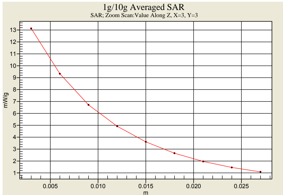
Body-Tissue-Simulating-Liquid 1900MHz
