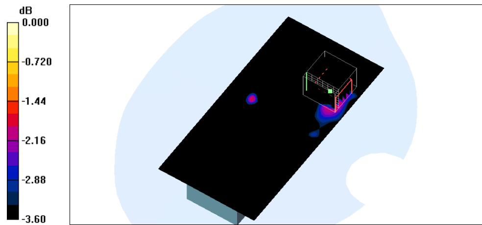
0 dB = 0.008mW/g
