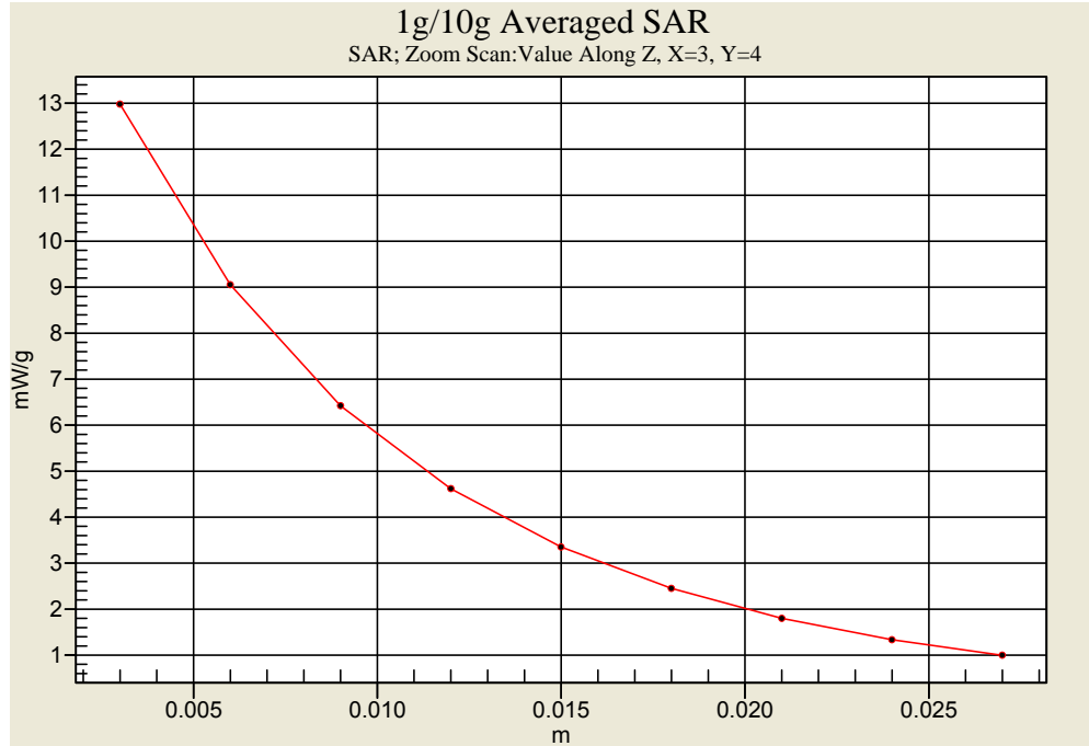
Head-Tissue-Simulating-Liquid 1900MHz
