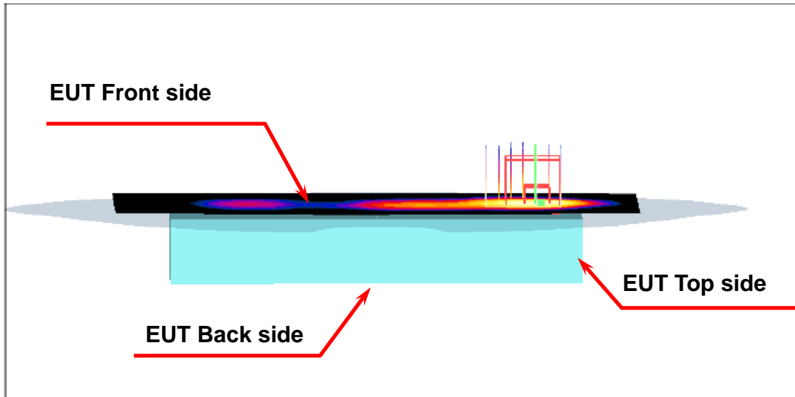
Figure 6. Body SAR Test Setup (Flat Section)
