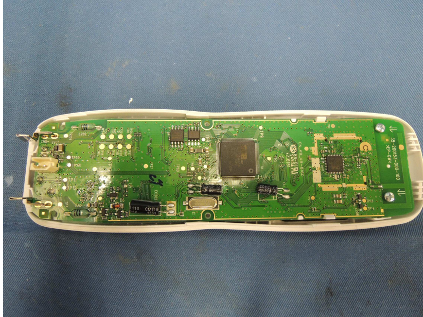
Handset assembly
