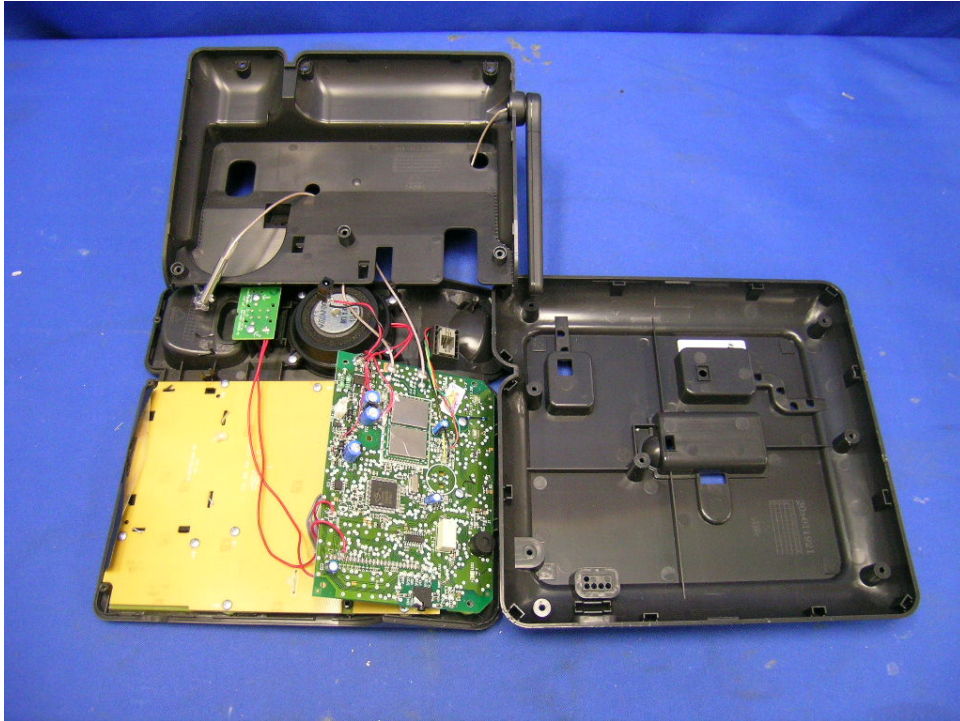
Deskset assembly (View 1)
