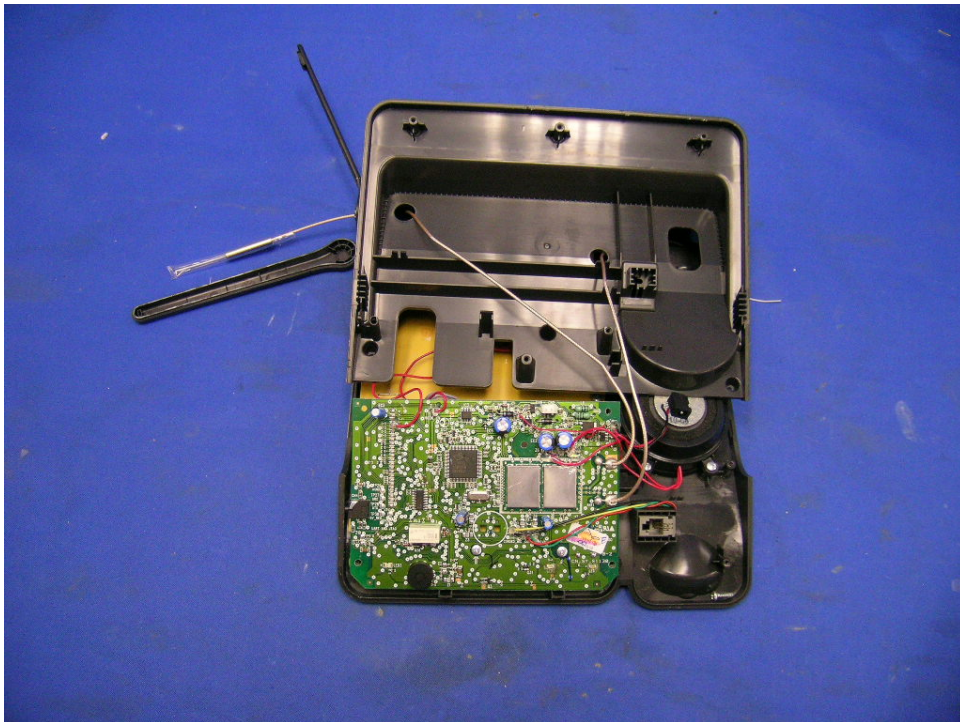
Deskset assembly (View 2)
