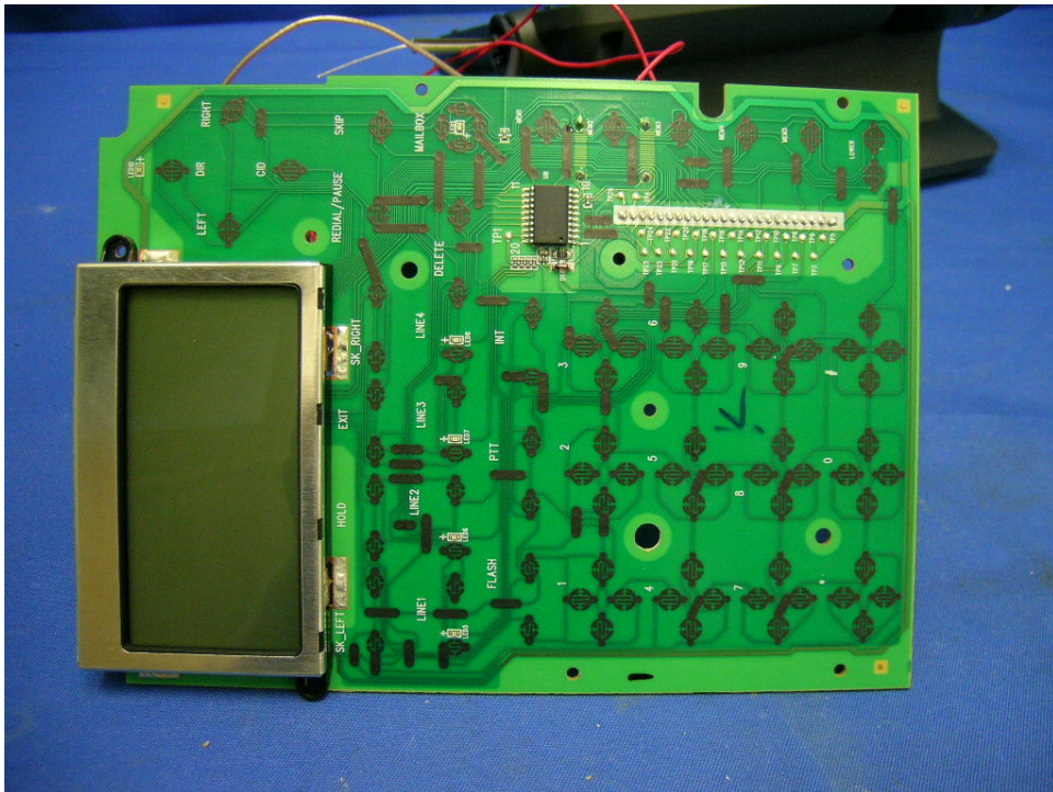
Deskset Keypad & Display View front side (View 1)
