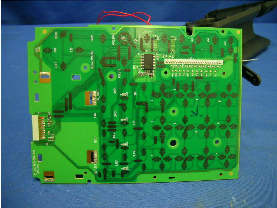
Deskset Keypad & Display View front side (View 2)
