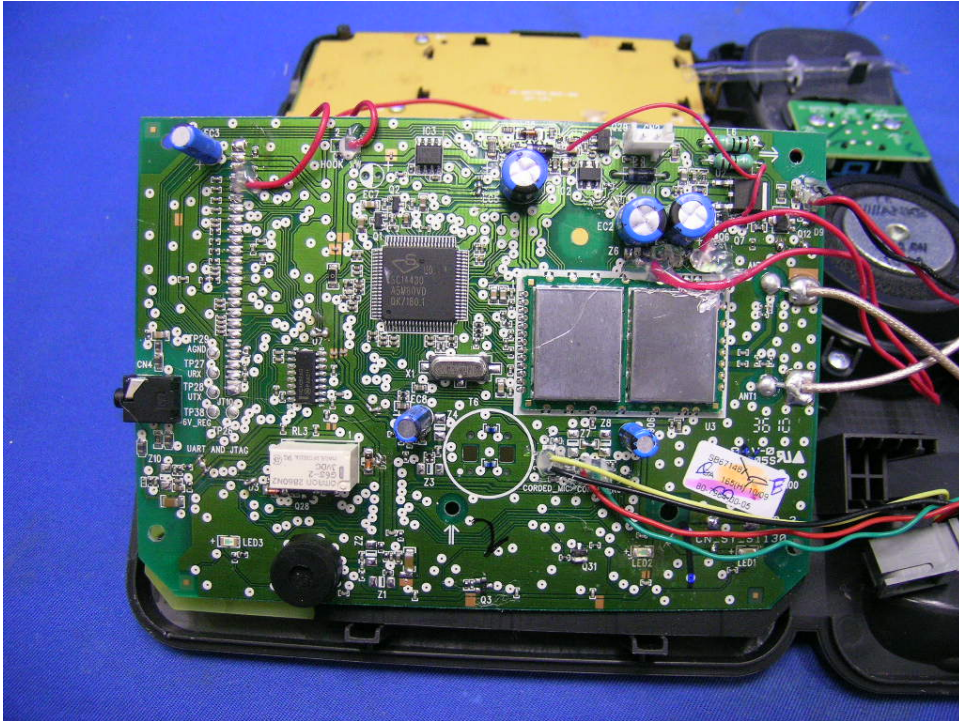
Deskset Main PCB comp side
