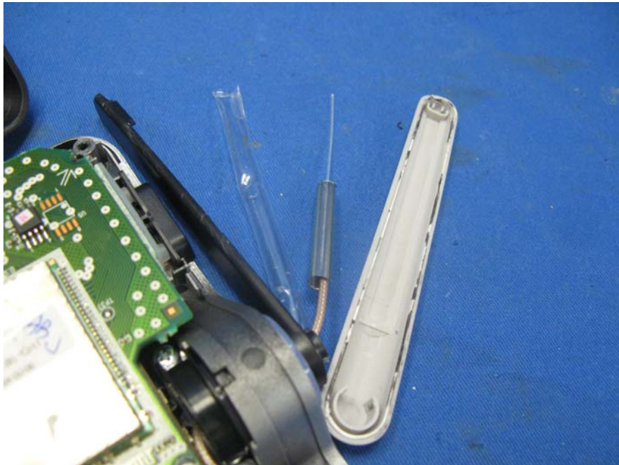
Base Unit DECT antenna 1
