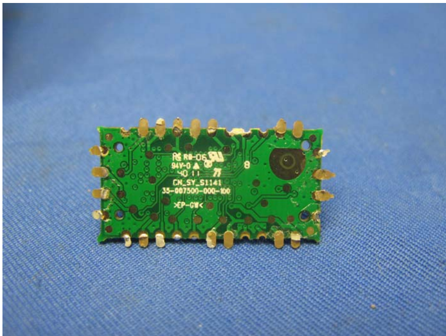
Base Unit Bluetooth RF module solder side
