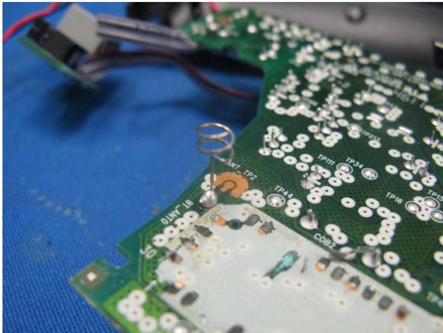
Base Unit Bluetooth antenna
