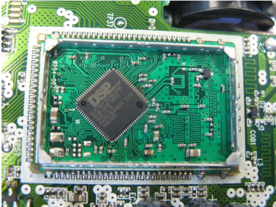
Base Unit DECT RF Module comp side
