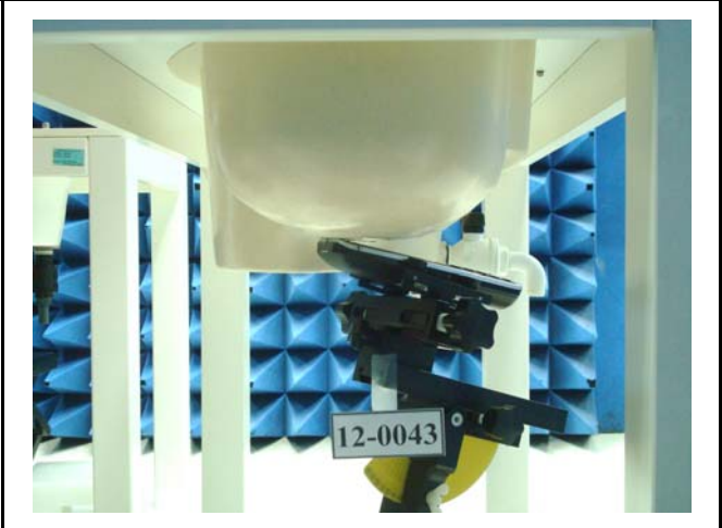
Figure 3. Right Head SAR Test Setup (Tilted)
