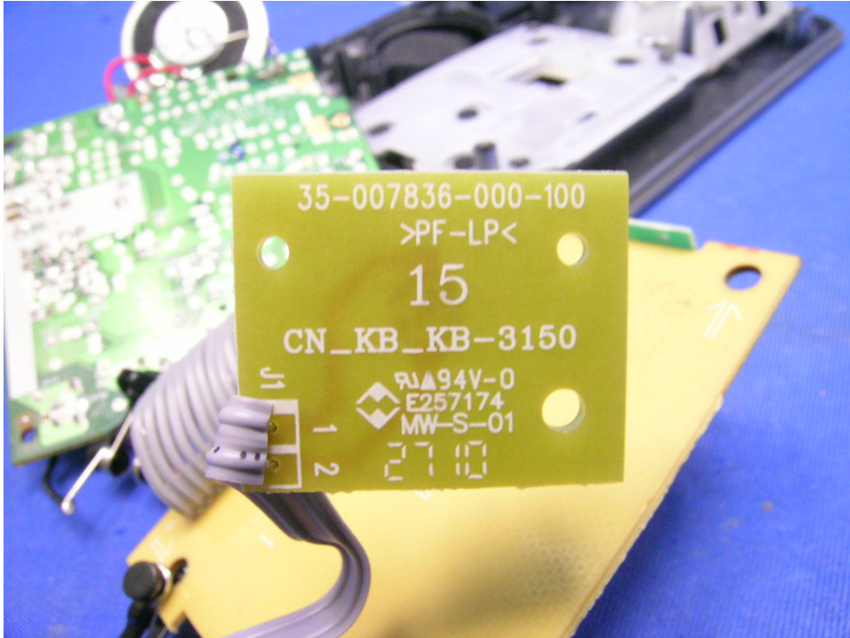
Base Unit Page Key Pad solder side
