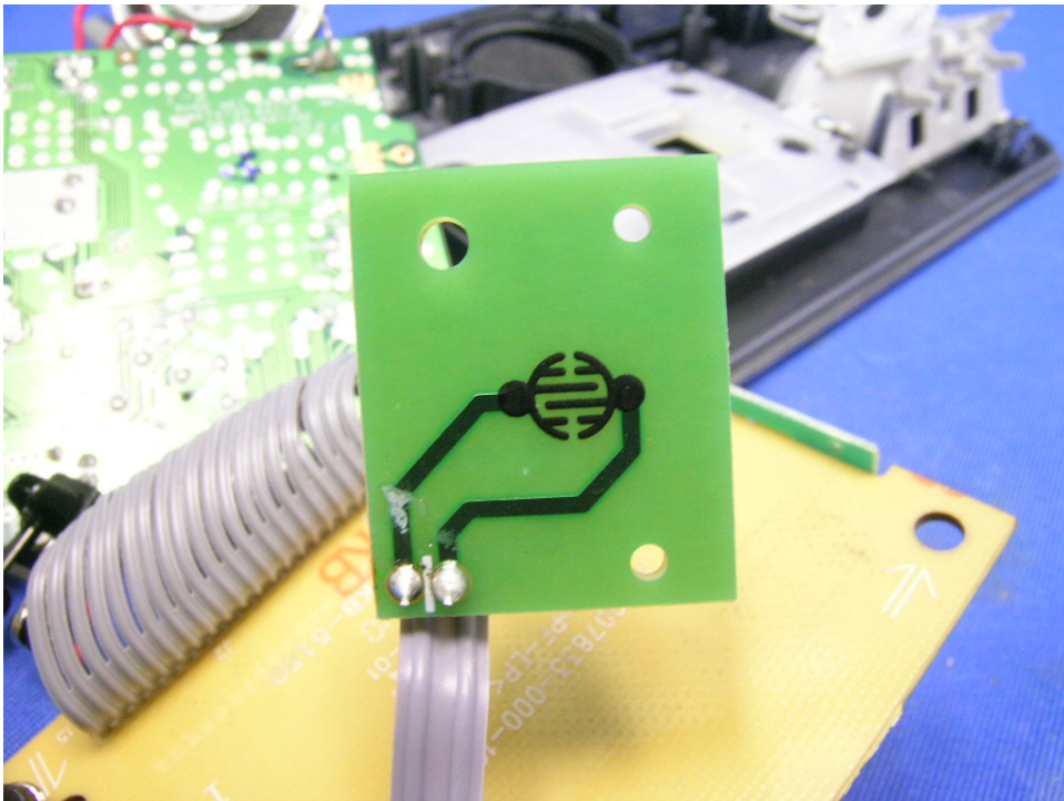
Base Unit Page Key Pad front side
