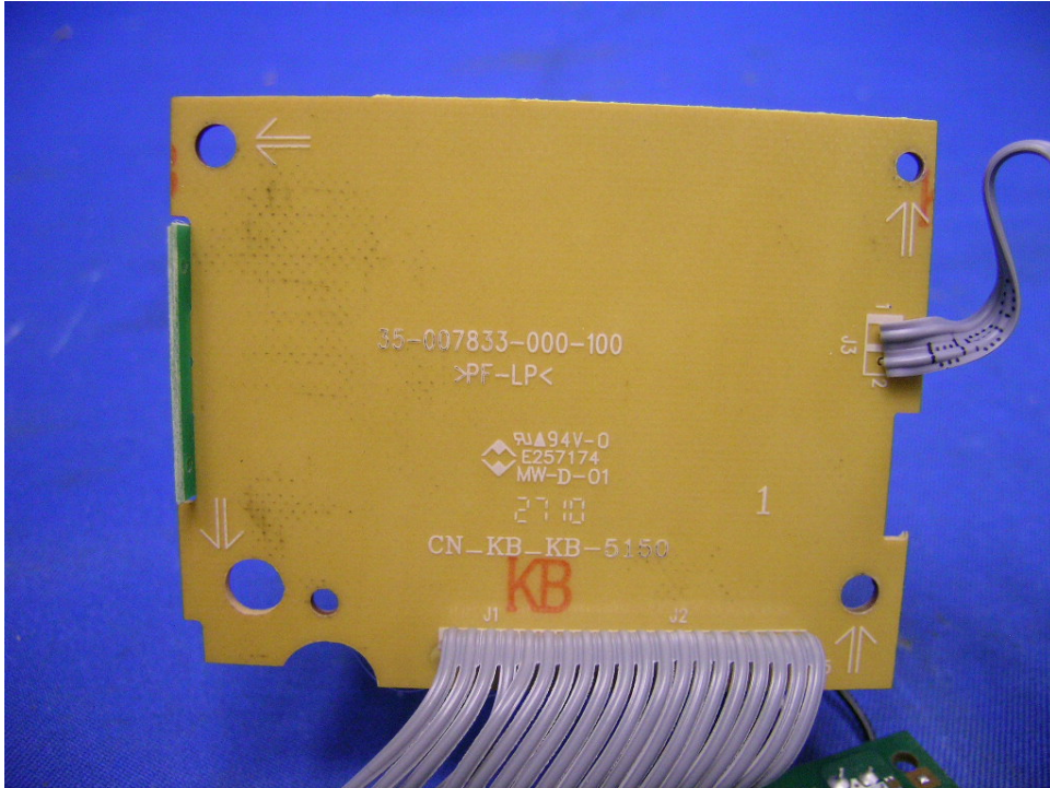
Base Unit DAM solder side
