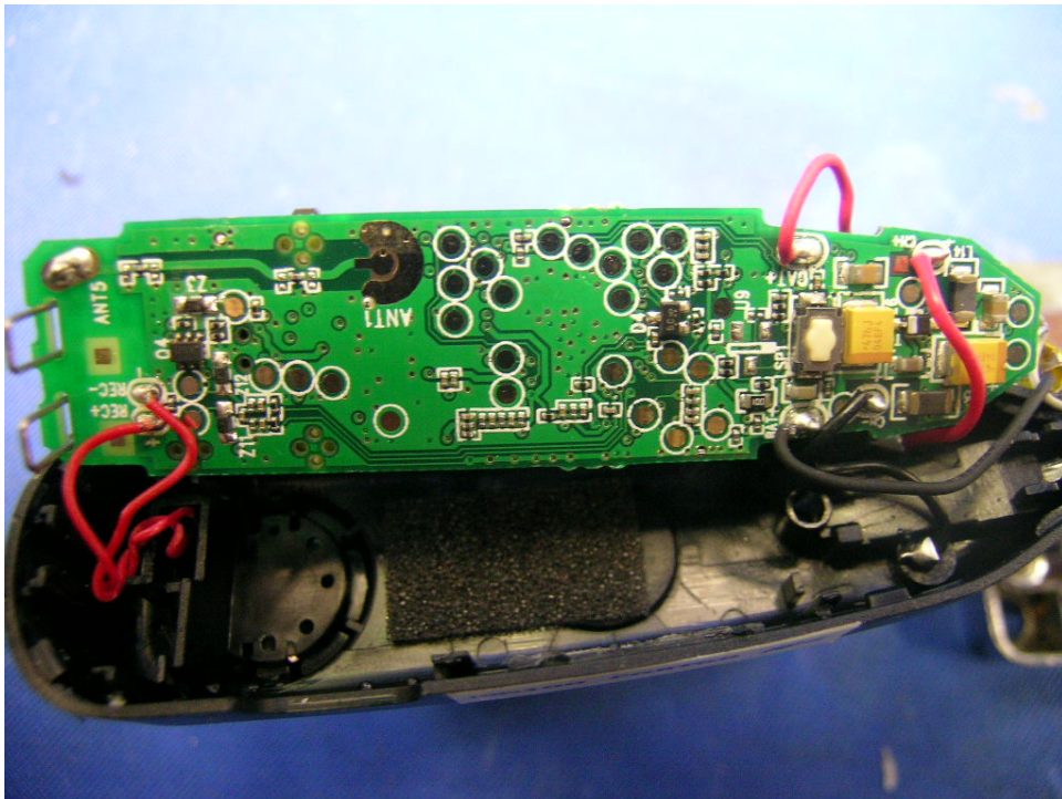
Headset Main PCB solder side (View 2)
