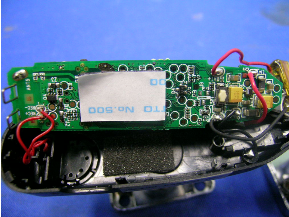
Headset Main PCB solder side (View 1)
