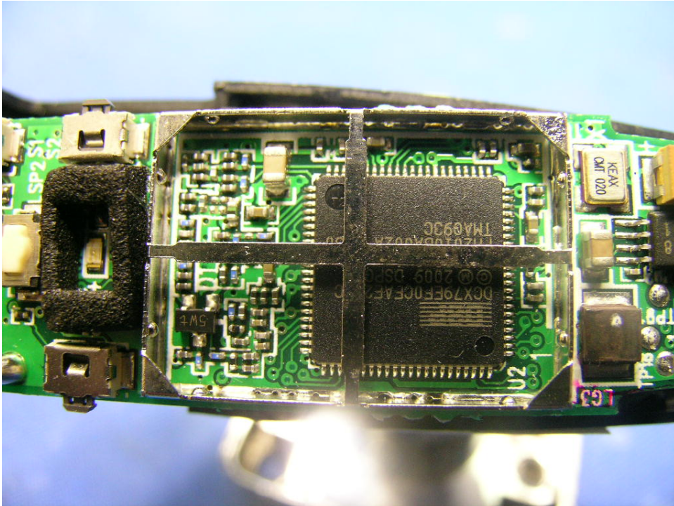
Headset Oscillator PCB comp side (View 1)
