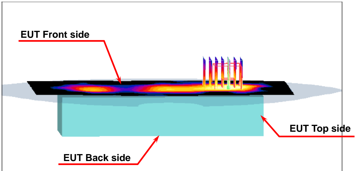
Figure 6. Body SAR Test Setup (Flat Section)
