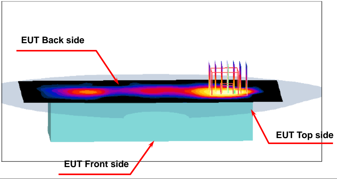
Figure 7. Body SAR Test Setup (Flat Section)
