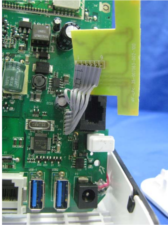
Base Unit Main PCB comp side (View 5)
