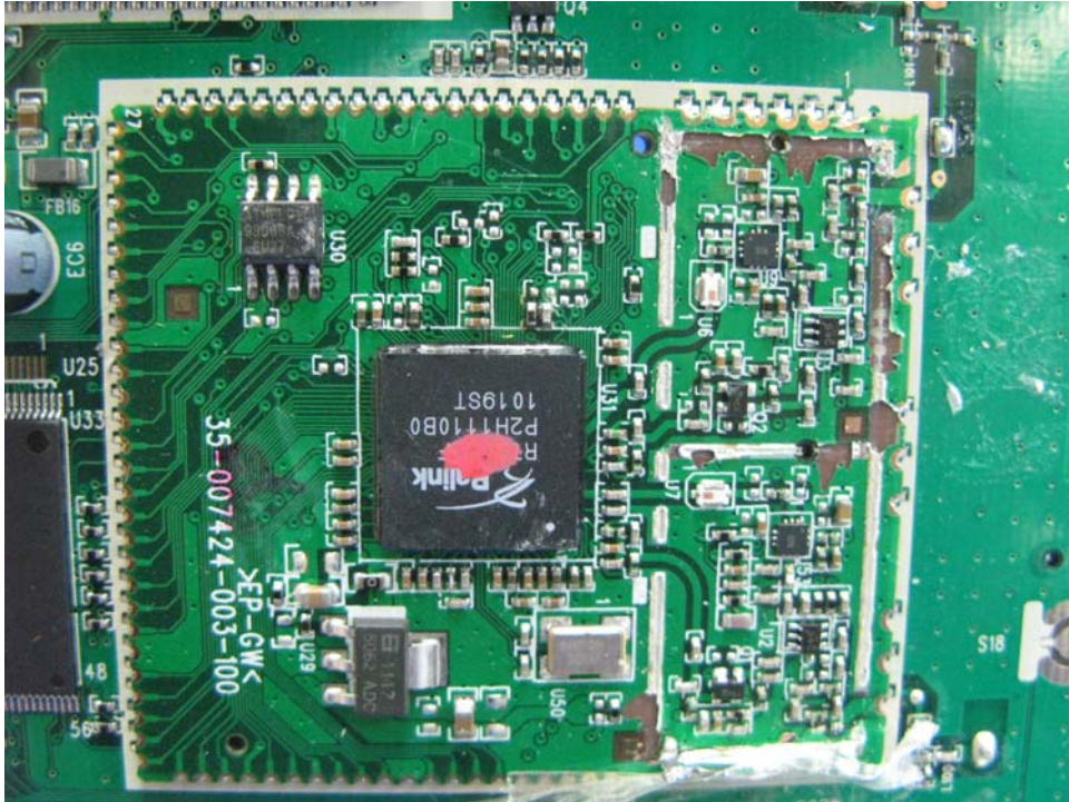
Base Unit WiFi front side
