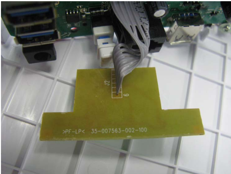
Base Unit LED Board rear side
