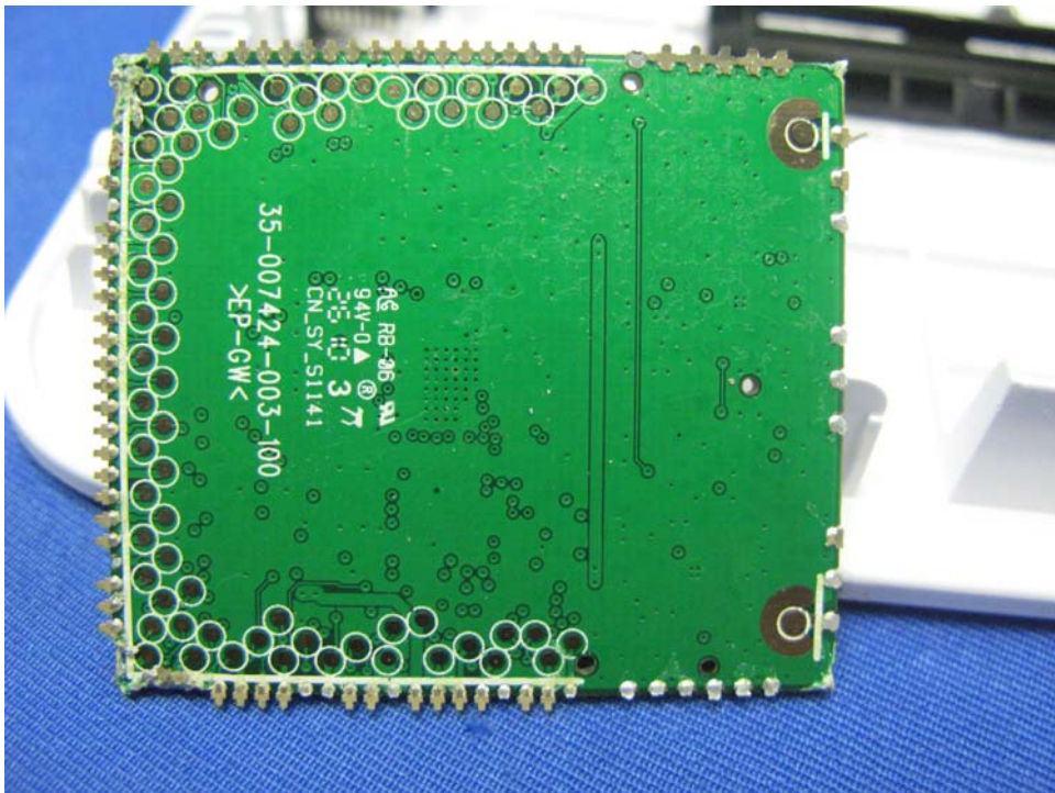
Base Unit WiFi rear side
