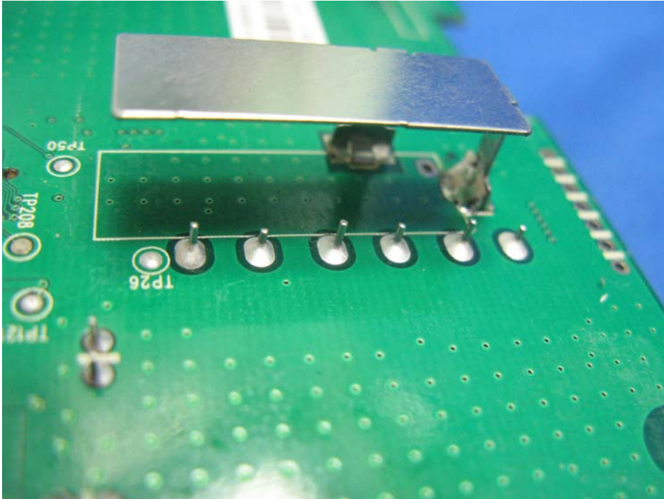
Base Unit Main PCB solder side (View 4)
