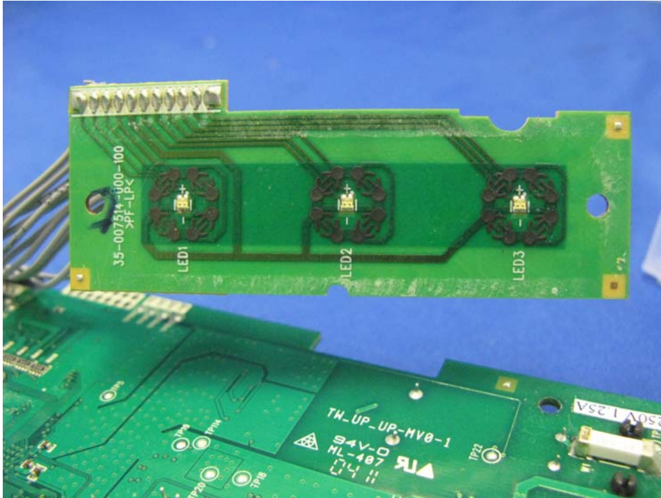
Base Unit LED and Keypad front side
