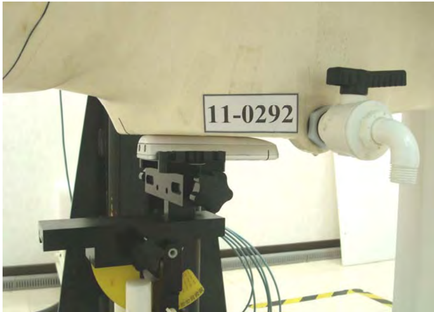
Figure 7. Body SAR Test Setup (Flat Section)
