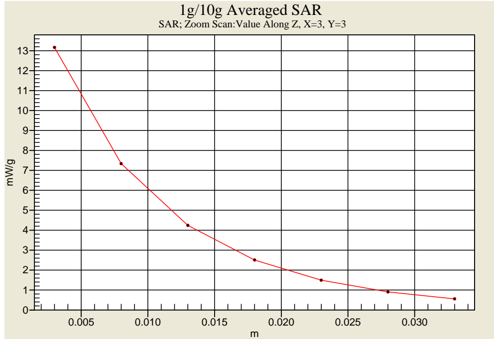
Head-Tissue-Simulating-Liquid 1900MHz
