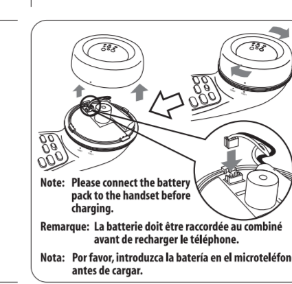
“Battery Charging Label” position
