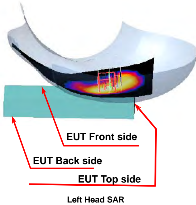
Figure 4. Left Head SAR Test Setup (Cheek)
