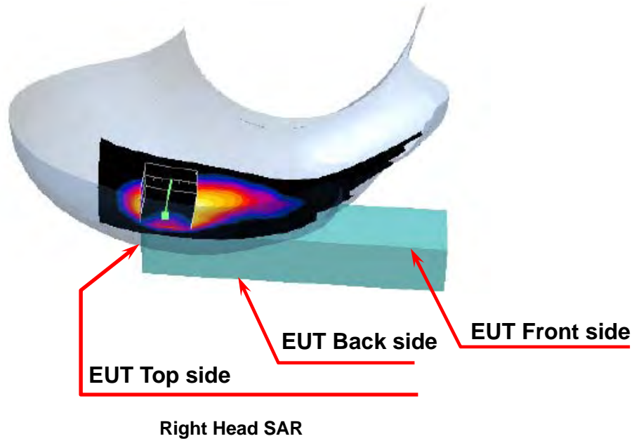
Figure 2. Right Head SAR Test Setup (Cheek)
