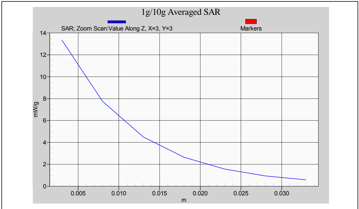
Body-Tissue-Simulating-Liquid 1900MHz
