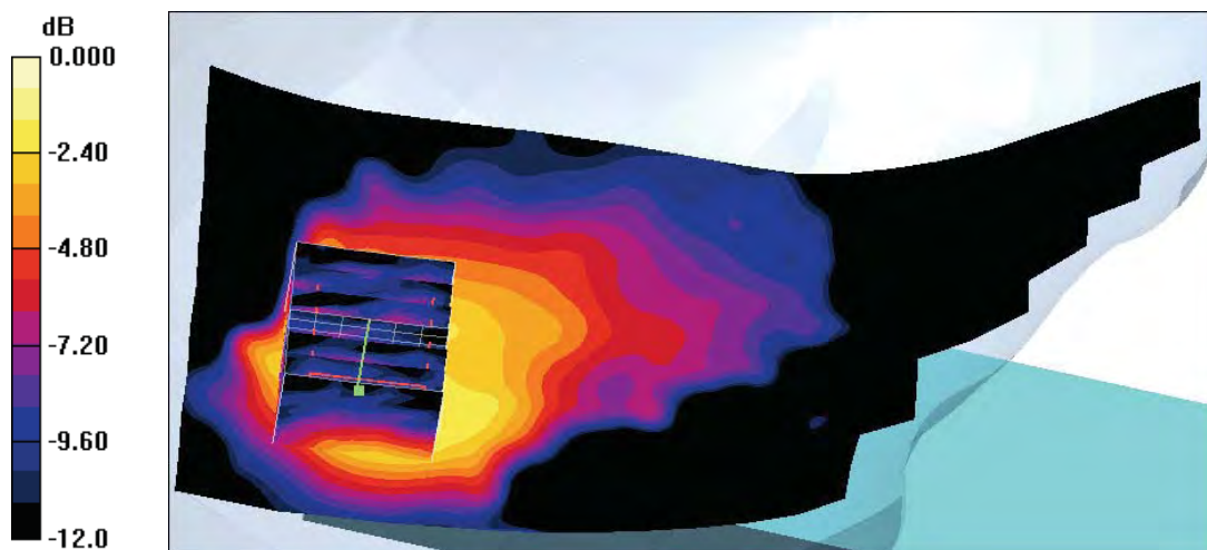
0 dB = 0.010mW/g
