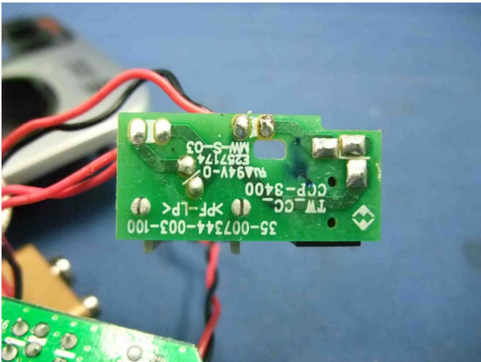
Base Unit Telephone Line Jack and AC Adaptor Jack rear side
