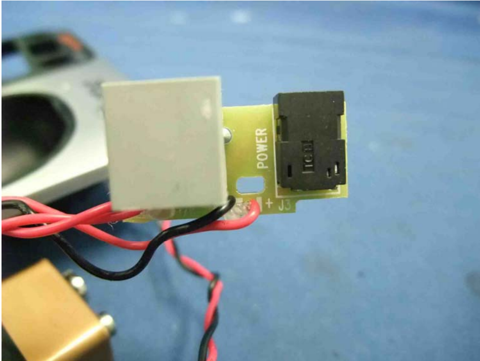
Base Unit Telephone Line Jack and AC Adaptor Jack front side
