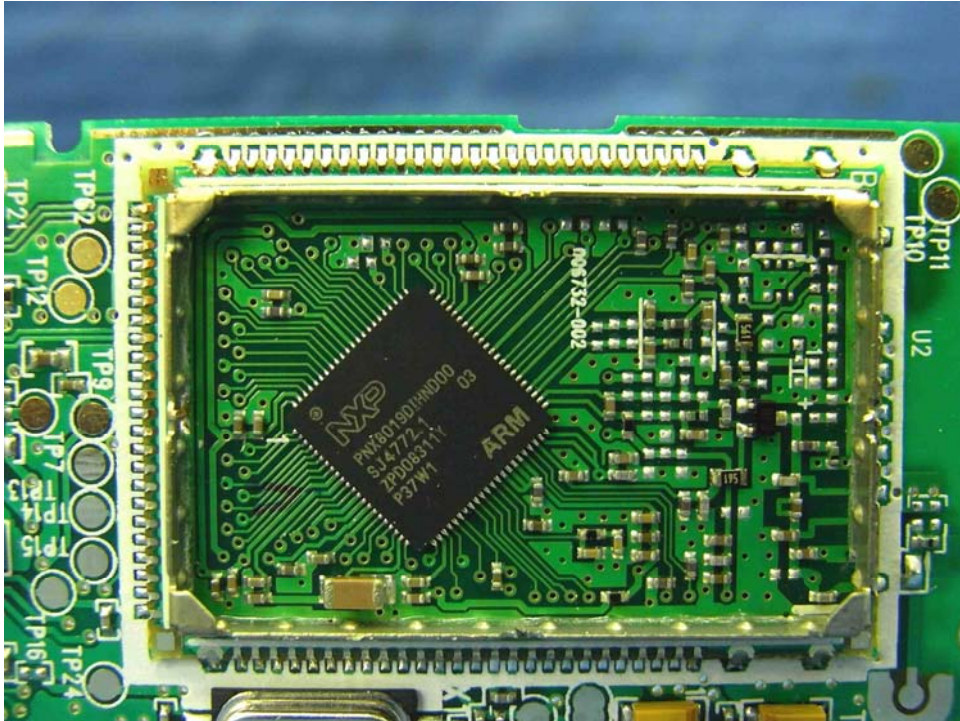
Handset Unit DECT RF Module PCB comp side
