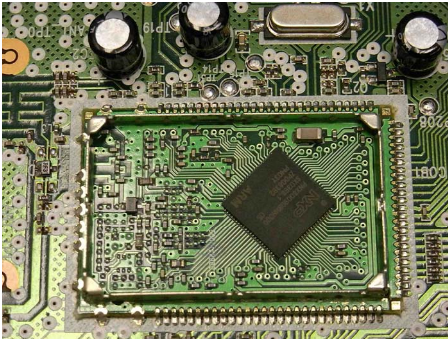
Base Unit RF Module PCB comp side
