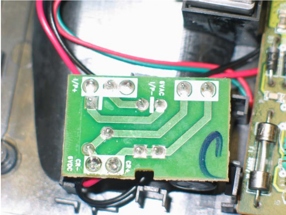
Base Unit Voltage Regulator rear side
