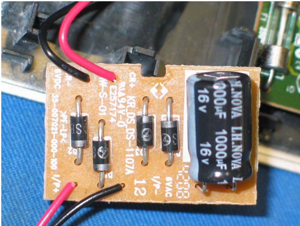
Base Unit Voltage Regulator front side
