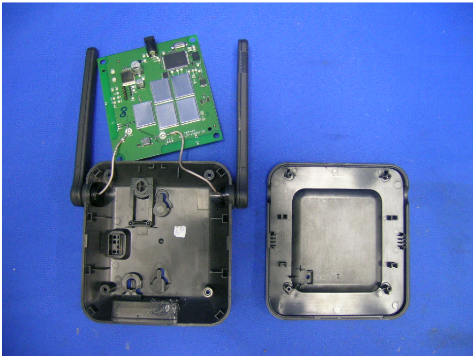
Repeater assembly (View 2)
