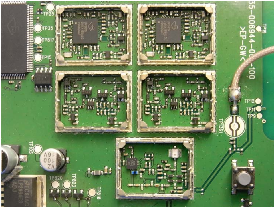
Repeater Oscillator PCB comp side
