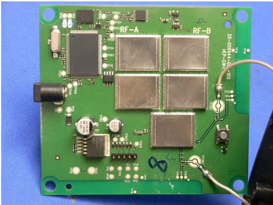
Repeater Main PCB comp side (View 2)
