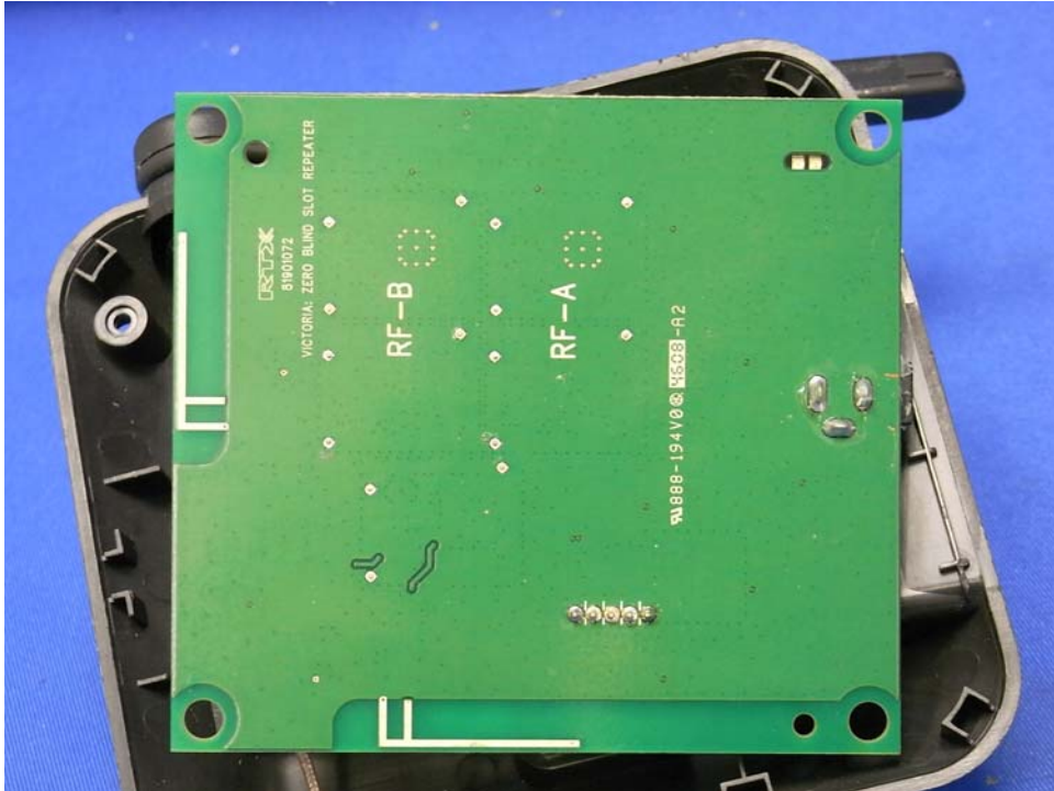
Repeater Main PCB solder side
