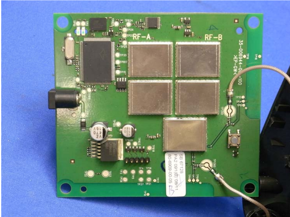
Repeater Main PCB comp side (View 1)
