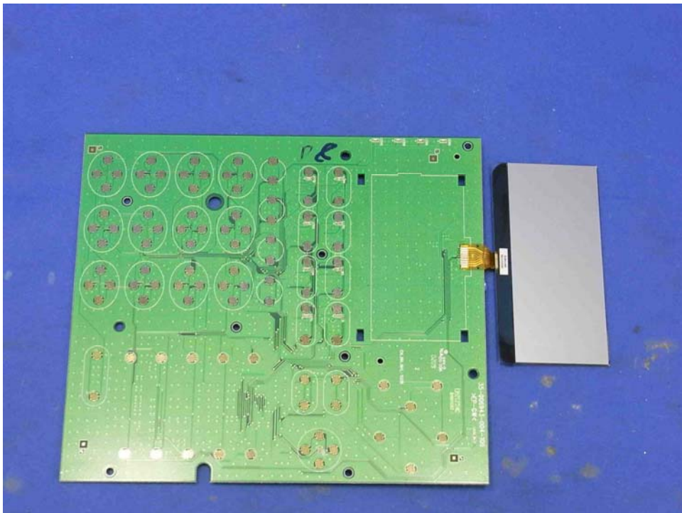
Base Unit LCD display solder side
