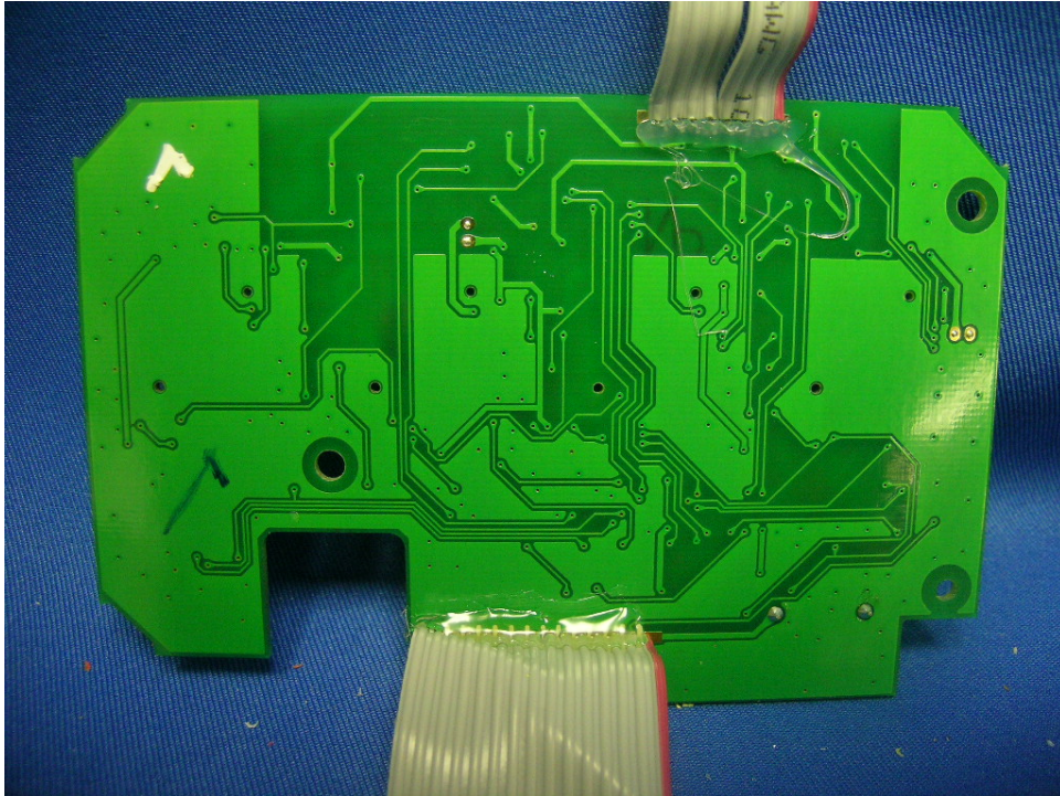
Base Unit Stutter Dial Tone PCB solder side
