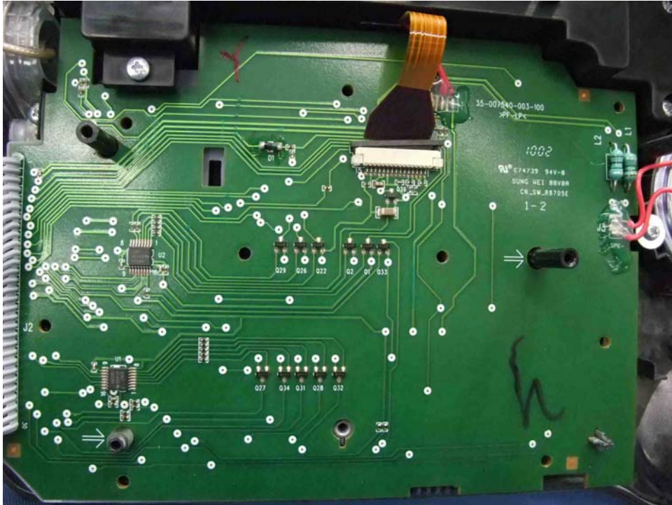
Base Unit Key Board front side (View 1)
