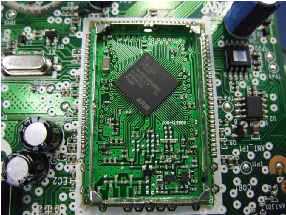
Base Unit DECT RF with Baseband Module PCB comp side
