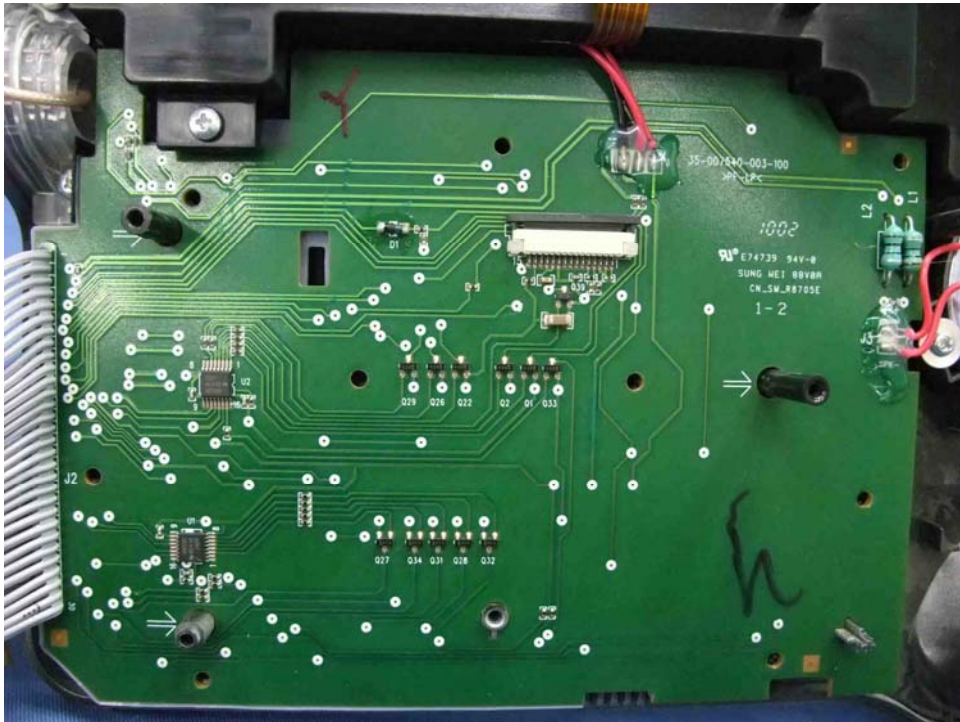
Base Unit Key Board front side (View 2)
