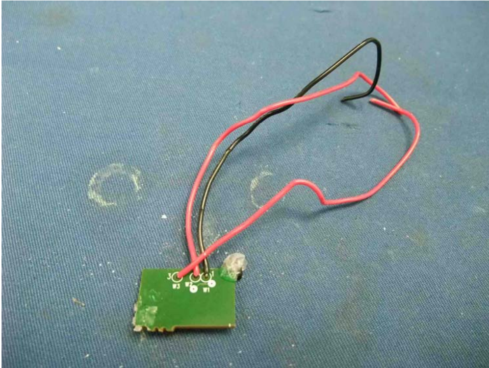
Base Unit Display Screen LED Board rear side
