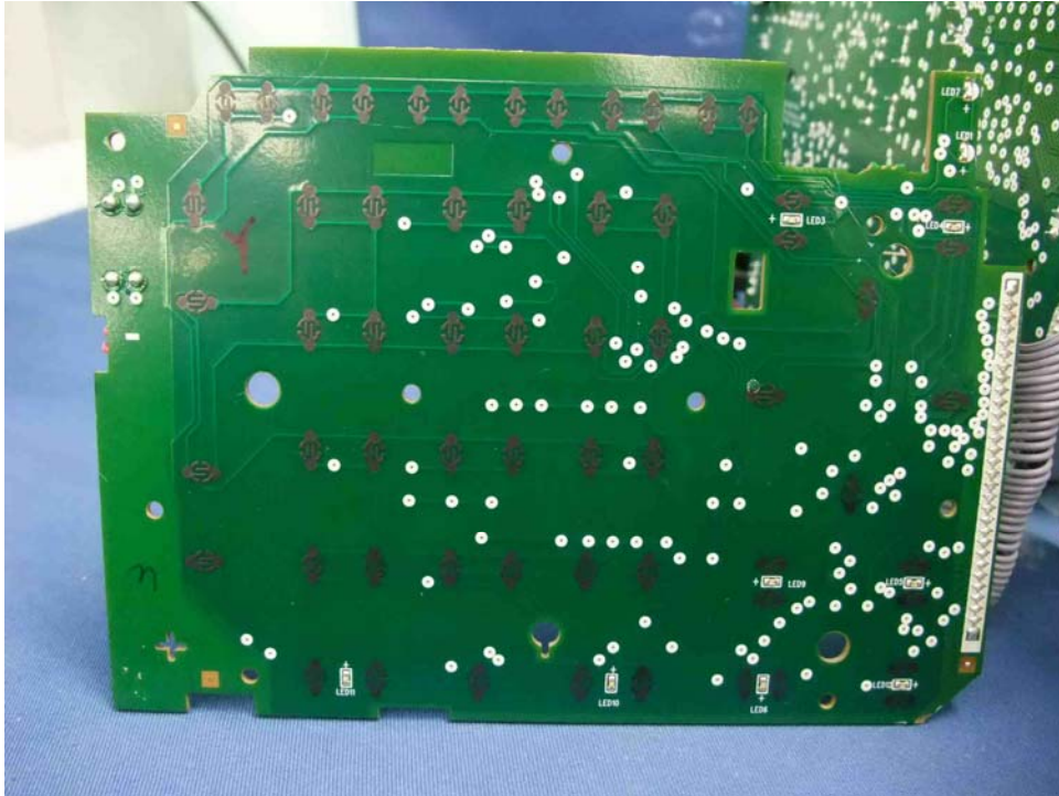
Base Unit Key Board rear side
