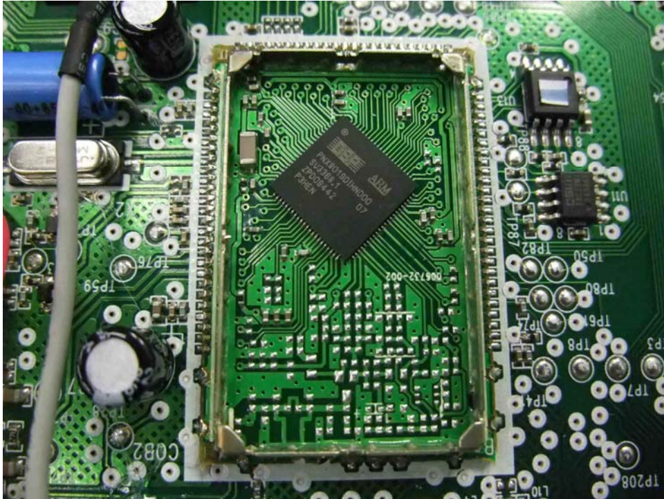
Base Unit DECT Baseband Module PCB comp side
