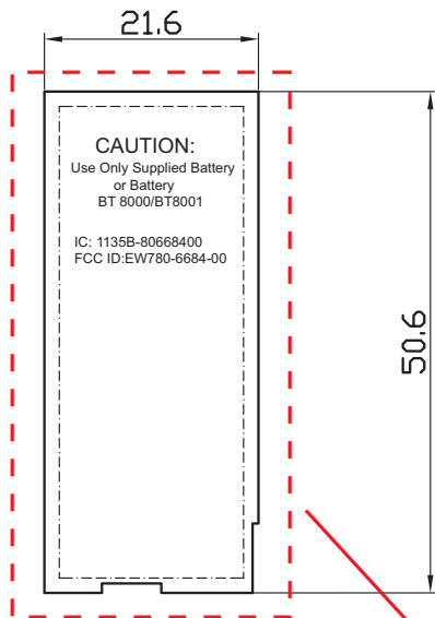
Caution Label
