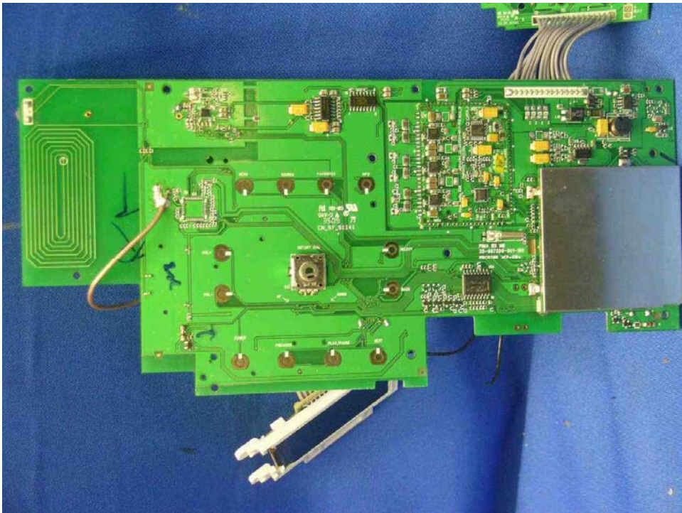
WiFi Internet Radio Main PCB front side (View 3)
