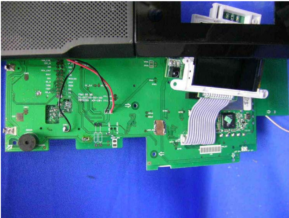
WiFi Internet Radio Main PCB rear side (View 3)
