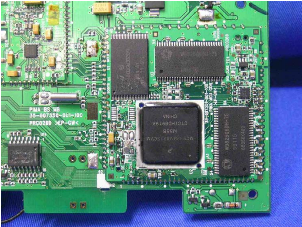
WiFi Internet Radio MCU front side (View 2)
