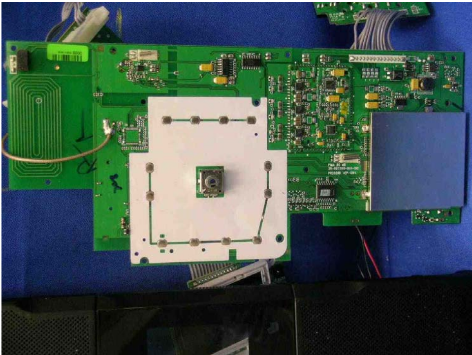
WiFi Internet Radio Main PCB front side (View 1)
