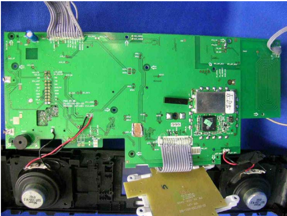
WiFi Internet Radio Main PCB rear side (View 1)
