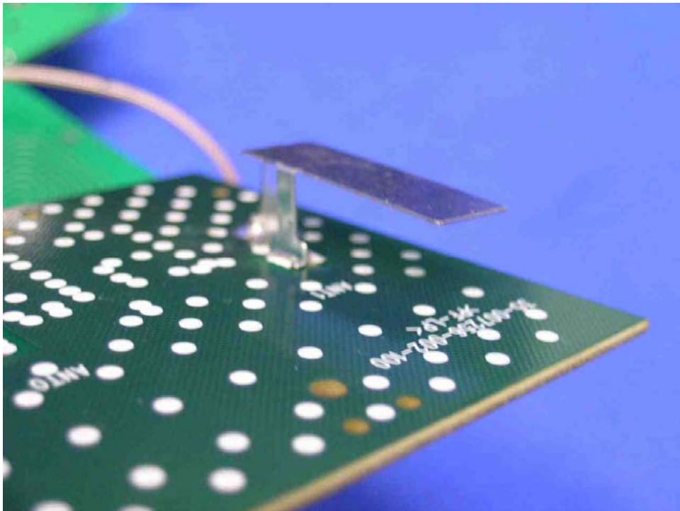
WiFi Internet Radio Antenna PCB rear side (View 2)
