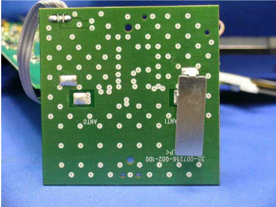
WiFi Internet Radio Antenna PCB rear side (View 1)
