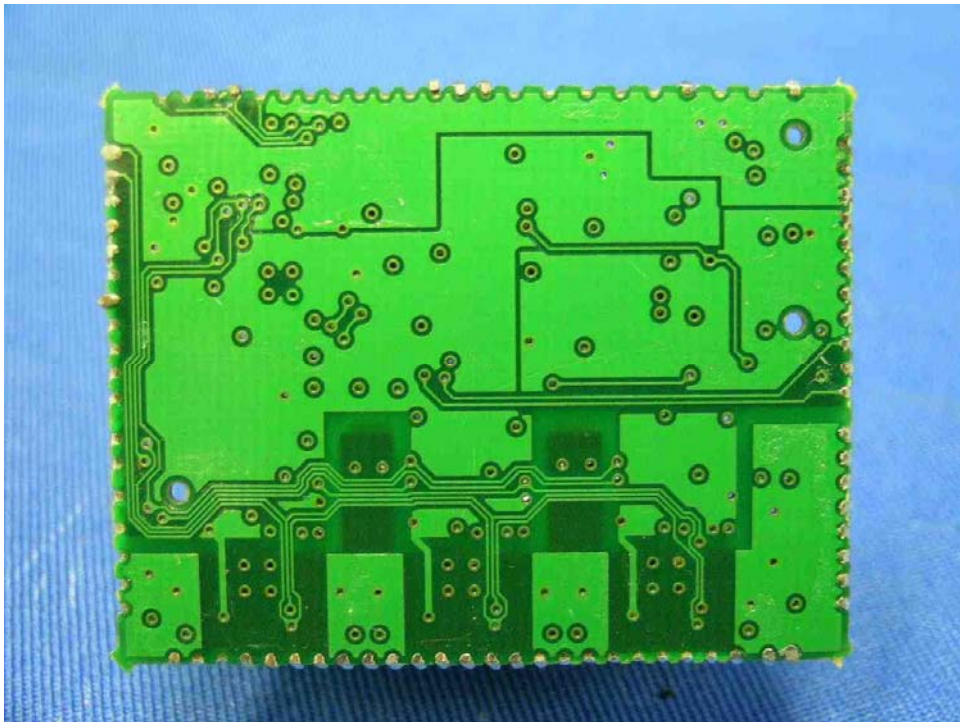
WiFi Internet Radio Audio COB rear side
