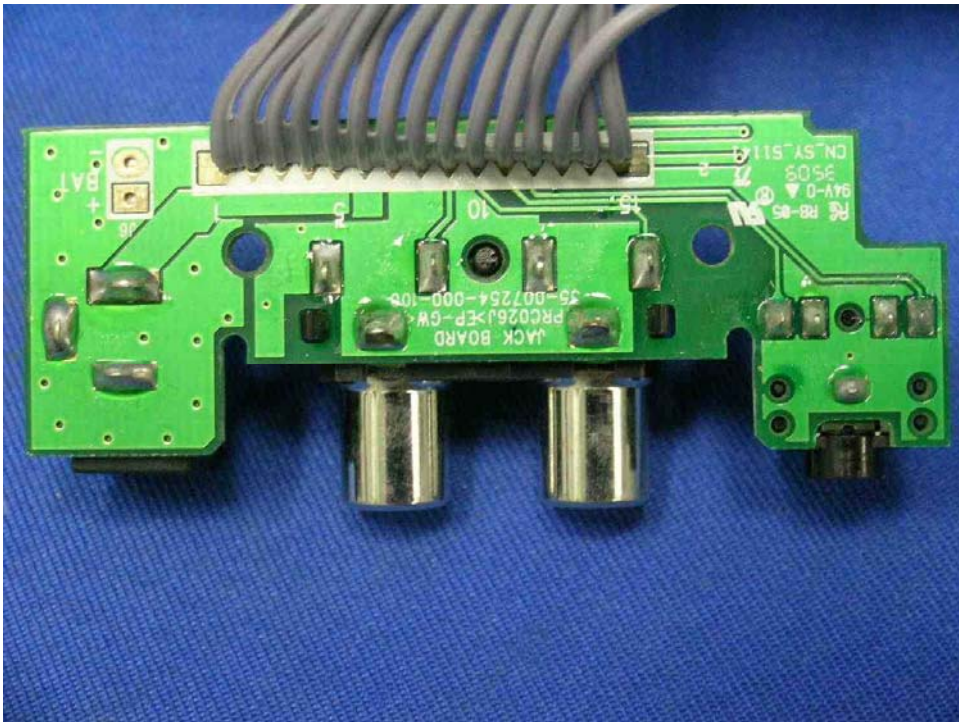
WiFi Internet Radio Jack PCB rear side
