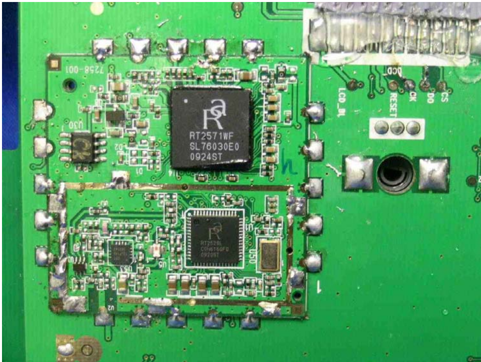
WiFi Internet Radio RF Module front side (View 2)
