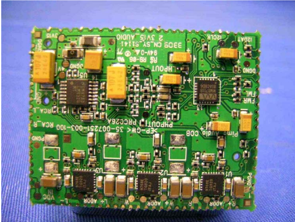
WiFi Internet Radio Audio COB front side
