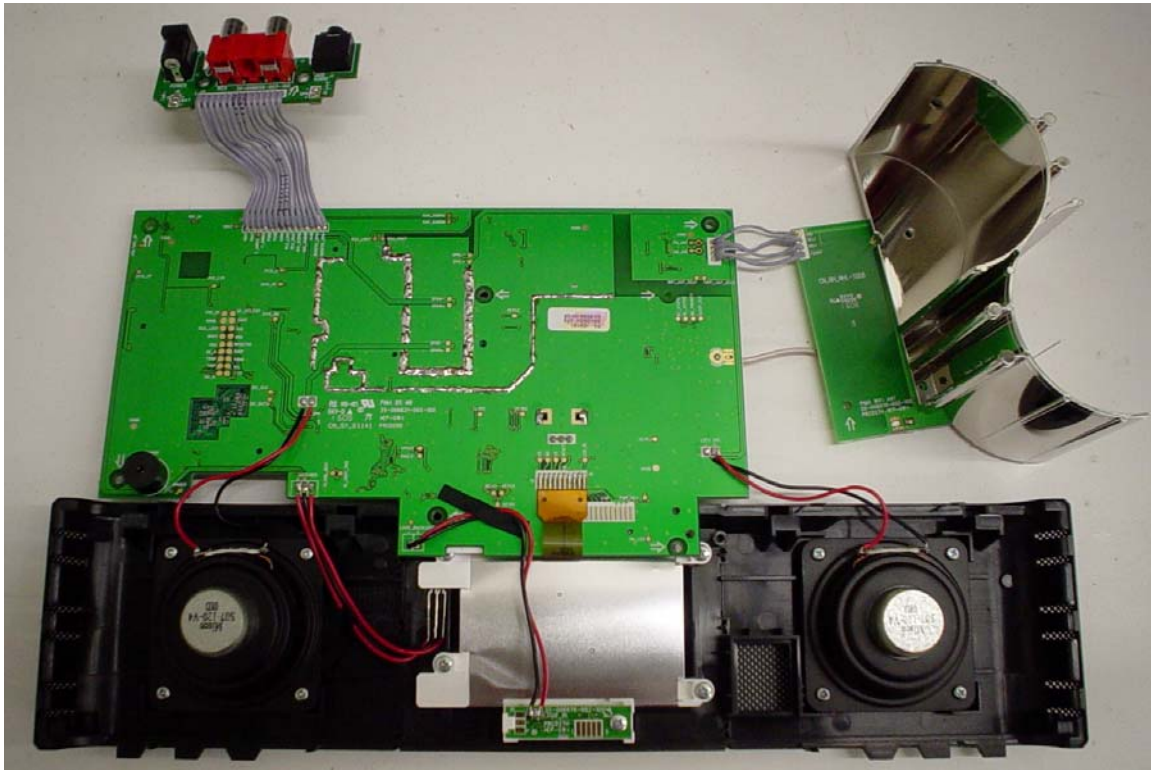
Vtech IS 9181 Circuit Board Bottom
