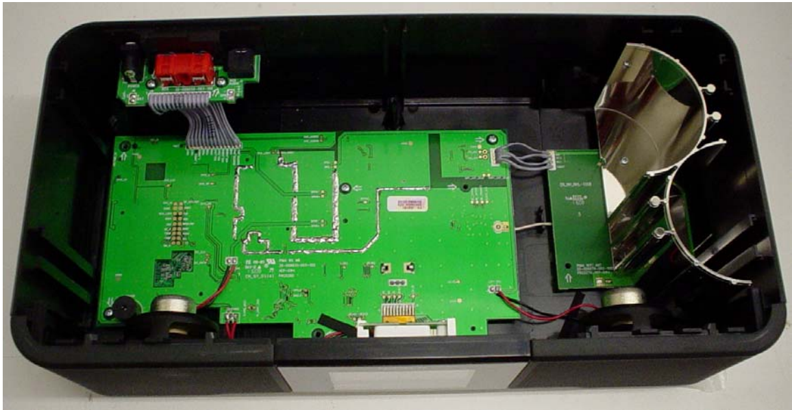
Vtech IS 9181 With Bottom Cover Removed
