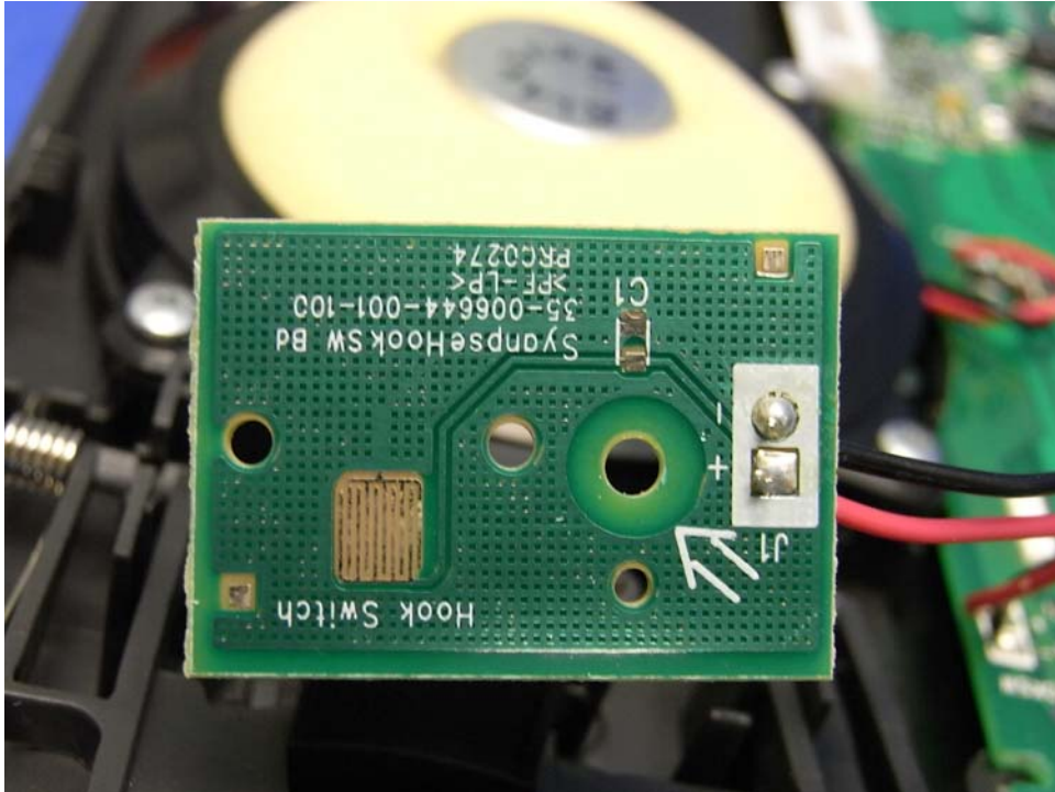
Deskset Hook switch PCB rear side
