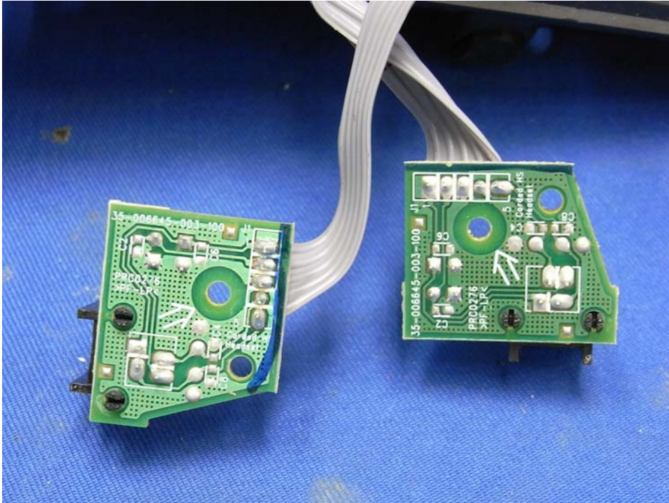
Deskset Handset & Headset Jack PCB solder side
