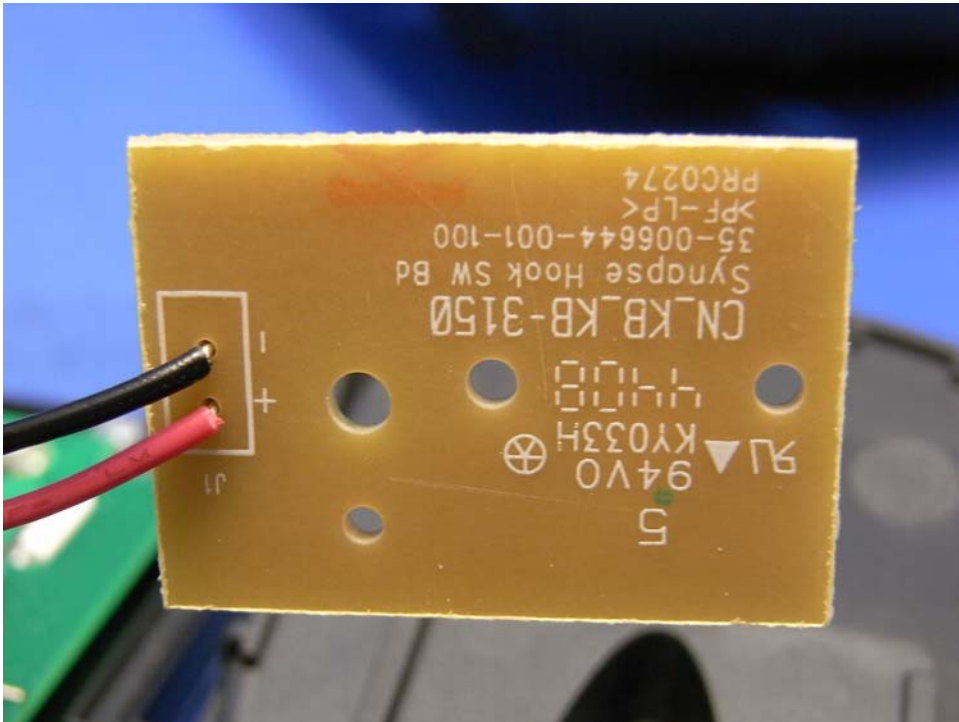
Deskset Hook switch PCB front side
