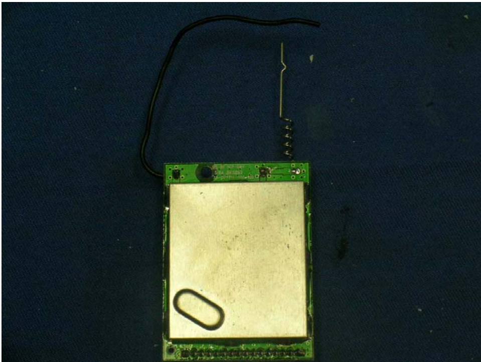
RF board with the shielding
