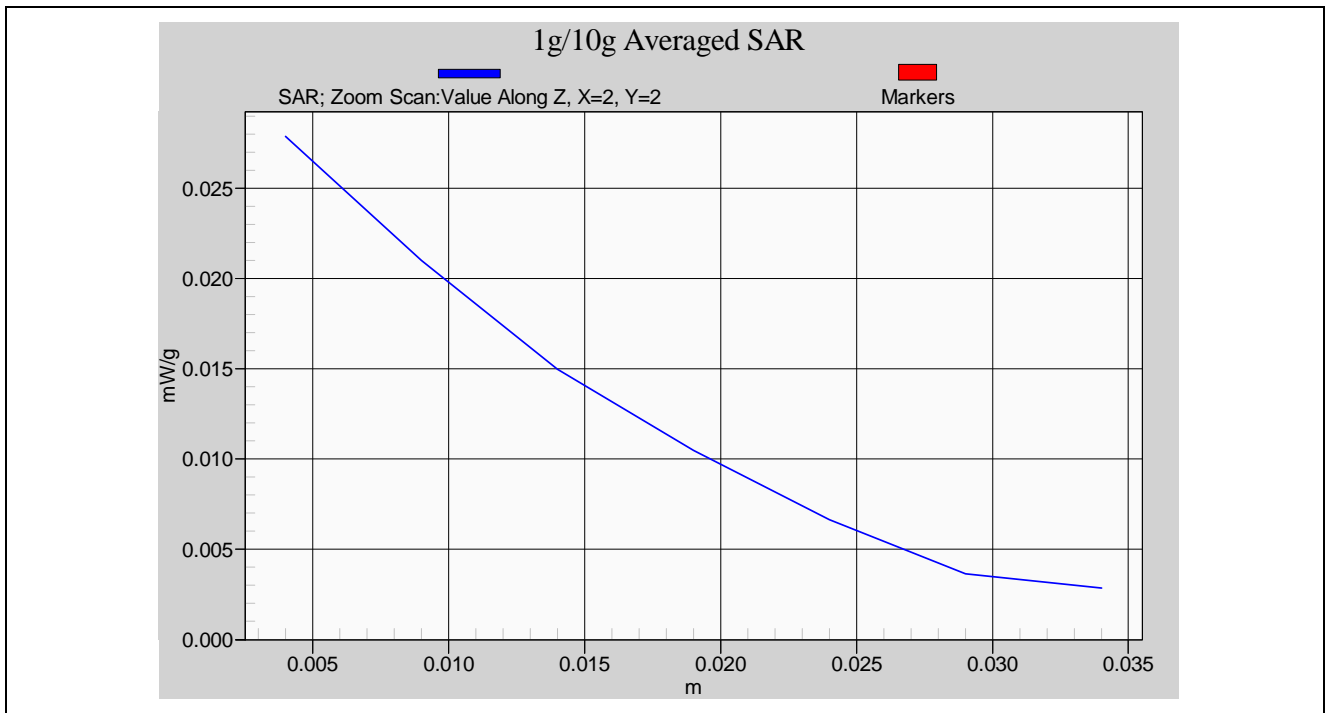
Head SAR Measurement _ Left Cheek CH2
