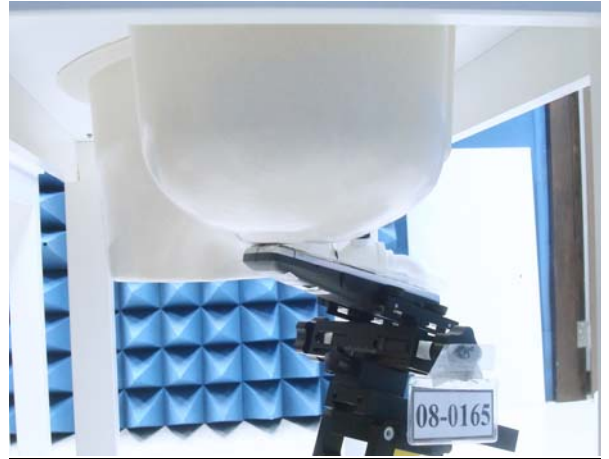
Figure 16. Right Head SAR Test Setup (Tilted)
