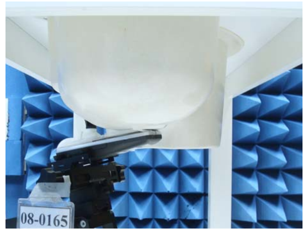
Figure 18. Left Head SAR Test Setup (Tilted)
