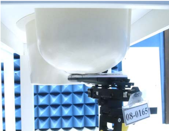
Figure 15. Right Head SAR Test Setup (Cheek)
