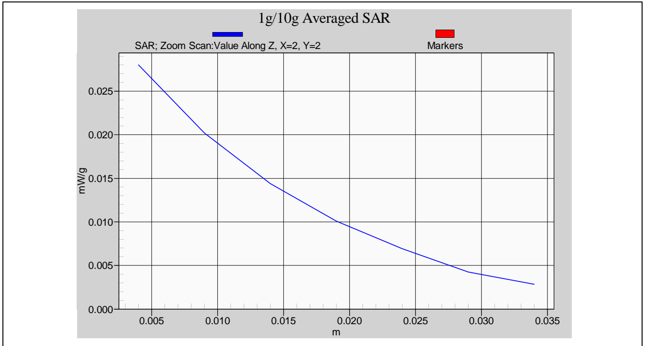
Head SAR Measurement _ Left Cheek CH4
