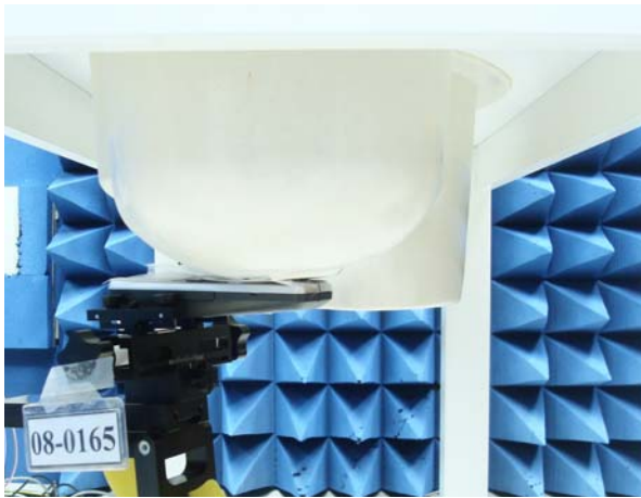
Figure 17. Left Head SAR Test Setup (Cheek)
