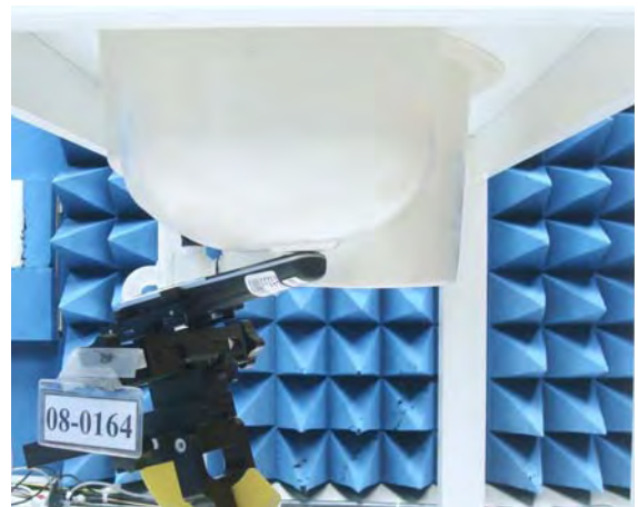
Figure 17. Left Head SAR Test Setup (Tilted)
