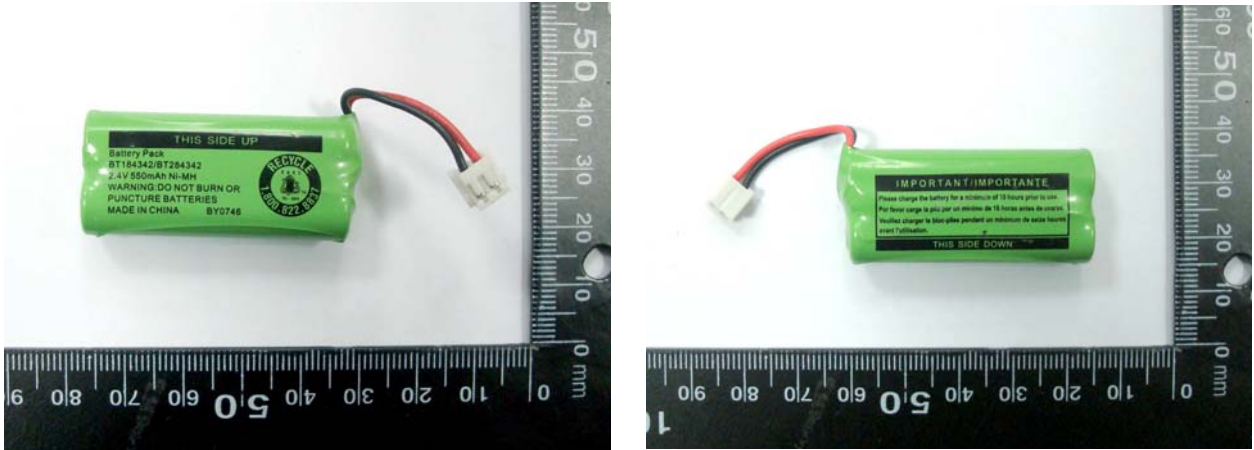
Figure 2. Battery (Ni-MH 2.4V , 550mAh)
