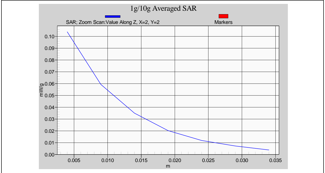
Body SAR Measurement _ Flat CH2
