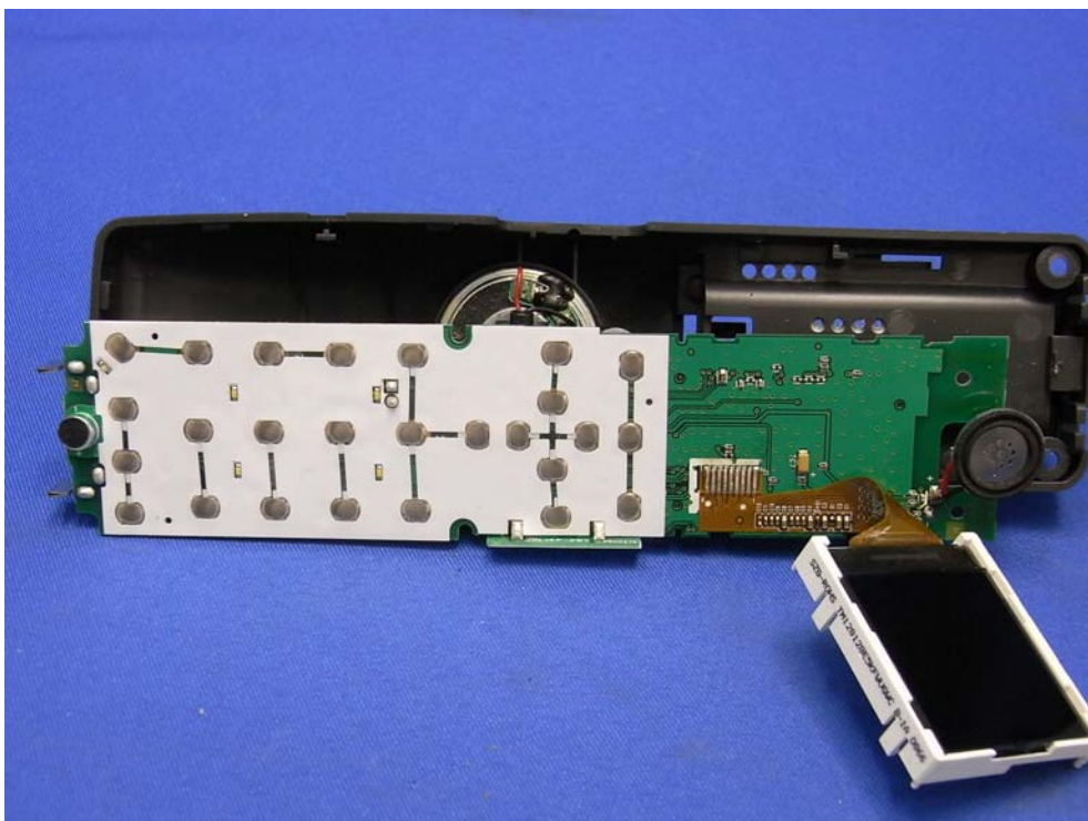
Handset Main PCB solder side (View 2)
