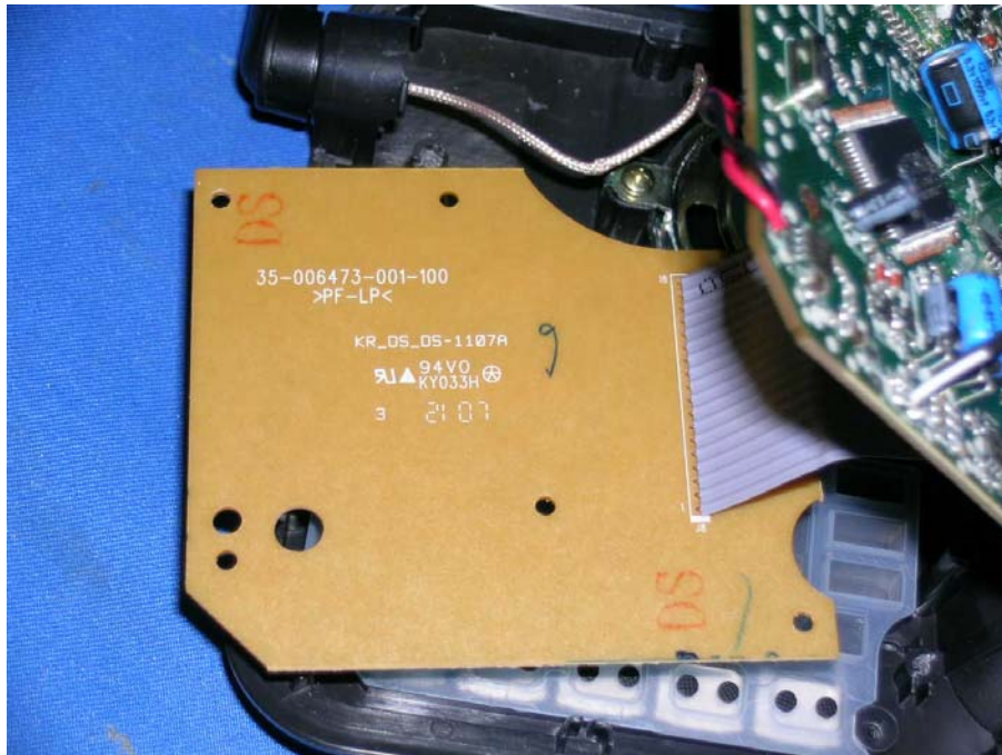
Base DAM rear side (View 1)
