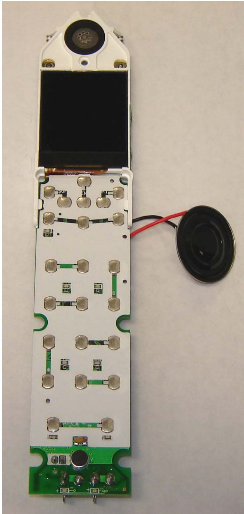
Vtech LS5145 Handset PCB
