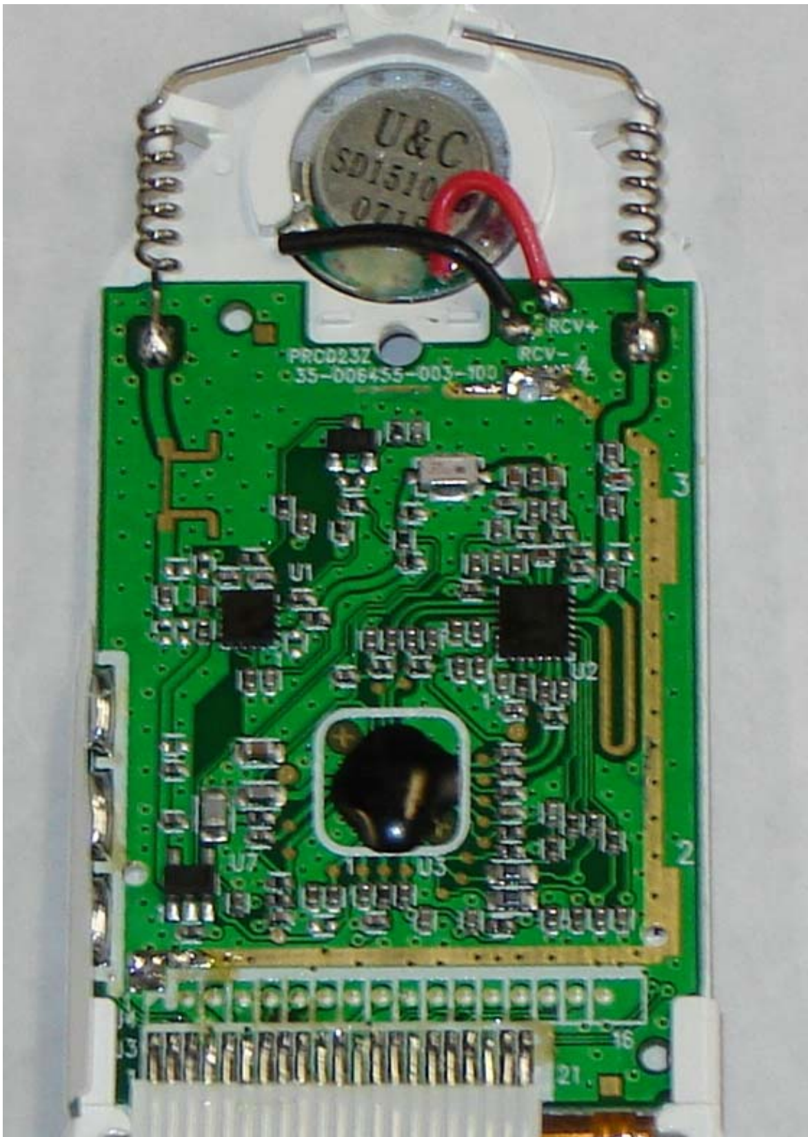
Vtech LS5145 Handset RF PCB
