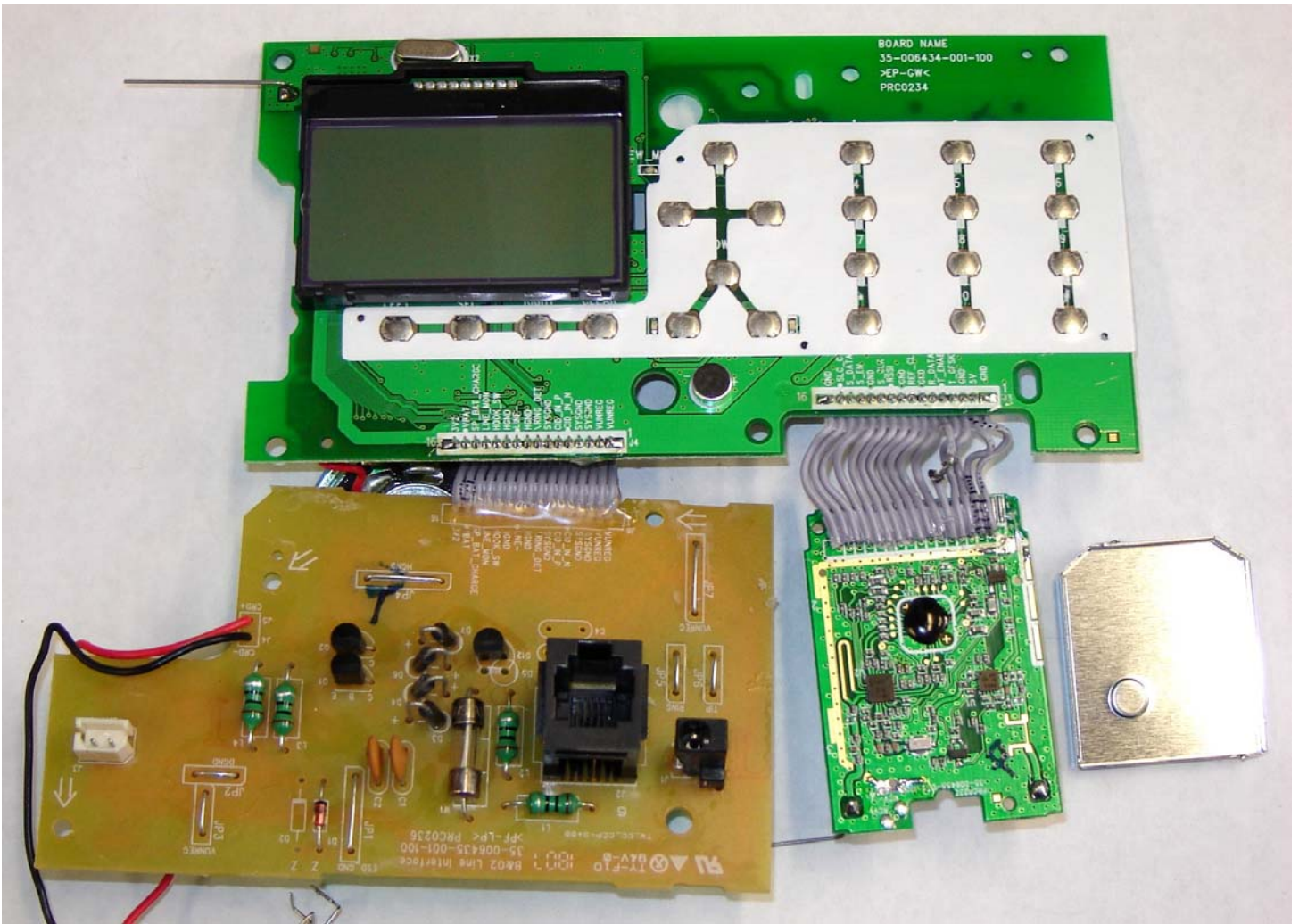
Vtech LS5145 Base PCB (without RF shield)
