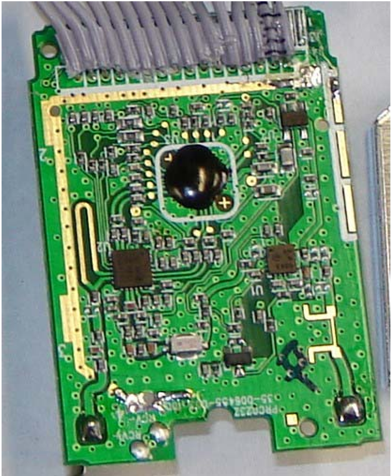
Vtech LS5145 Base RF PCB
