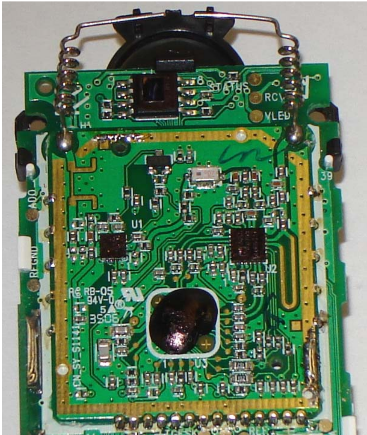
AT&T EP5632 Handset PCB
