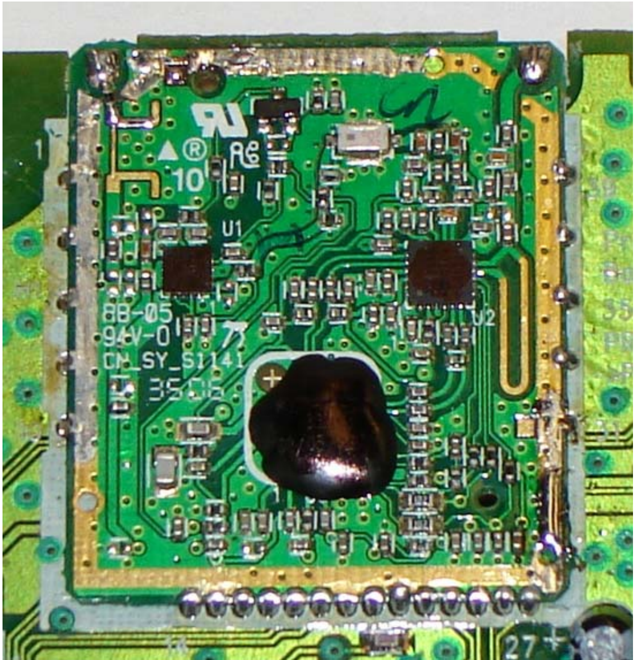
AT&T EP5632 Base RF
