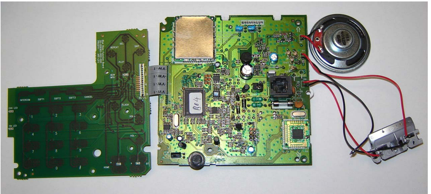
AT&T EP5632 Base PCB
