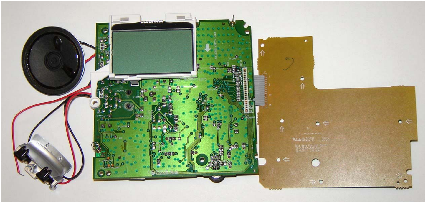
AT&T EP5632 Base PCB
