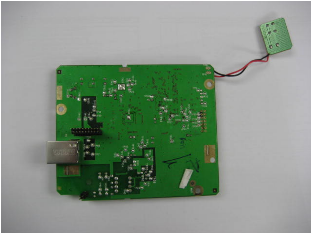
Figure 4: PCB - Back
