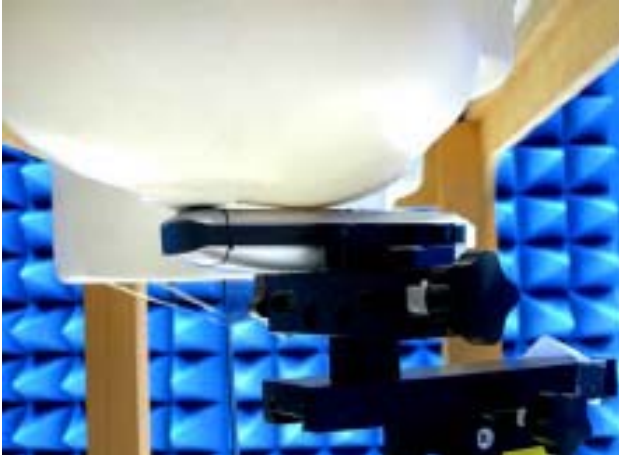
Figure 16. Right Head SAR Test Setup (Cheek)
