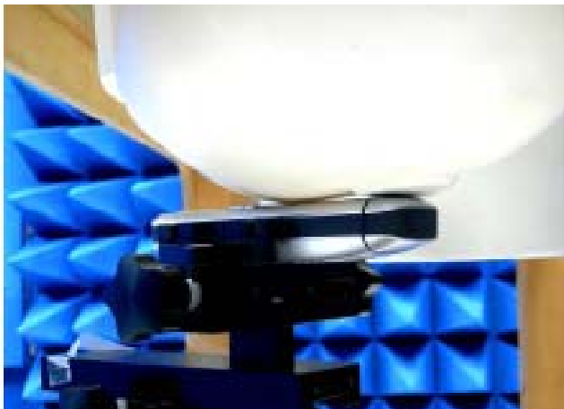
Figure 18. Left Head SAR Test Setup (Cheek)
