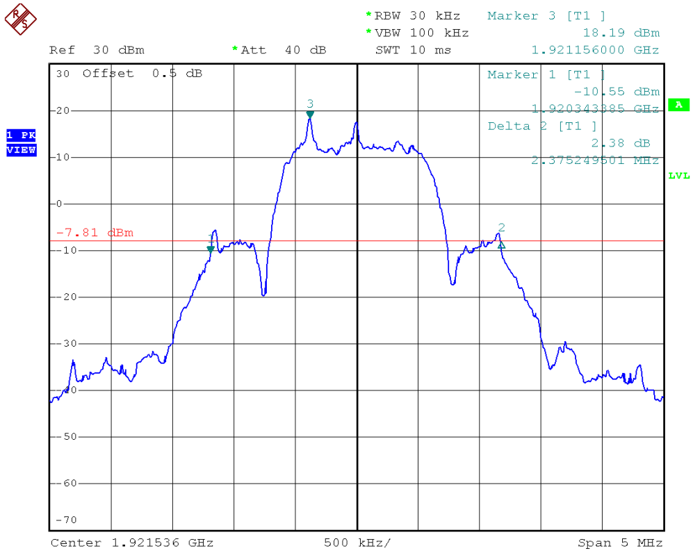
Plot 1A. Lowest Channel 26dB Emission Bandwidth (Traffic Carrier)
