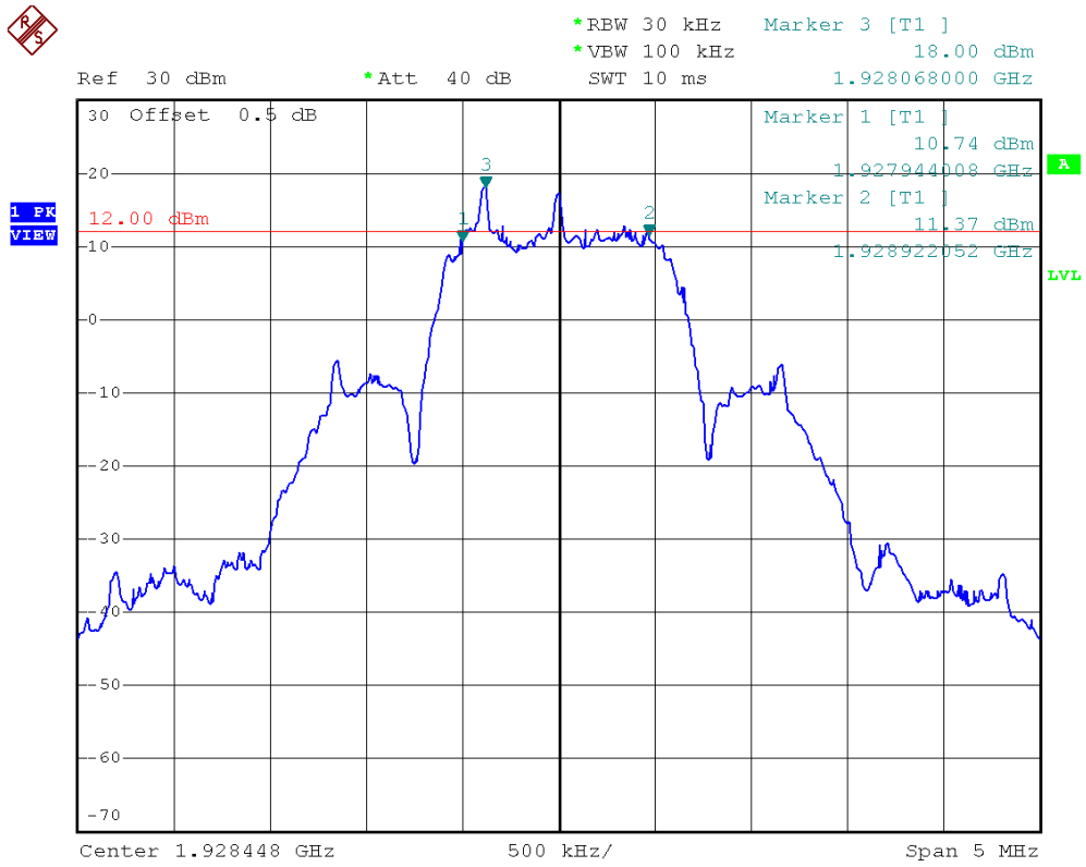
Plot 1E. Highest Channel Test Frequency at -6dB points (Traffic Carrier)
