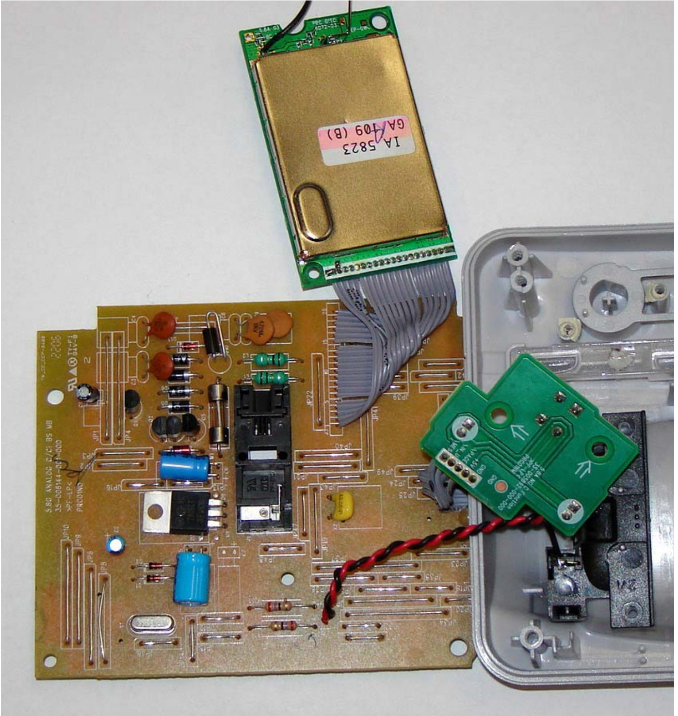
Vtech ia5823 Base PCB
