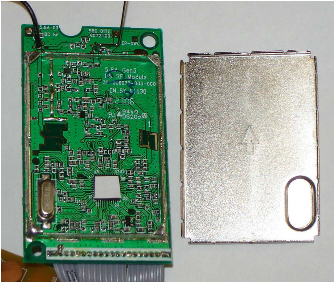
Vtech ia5823 Base RF PCB
