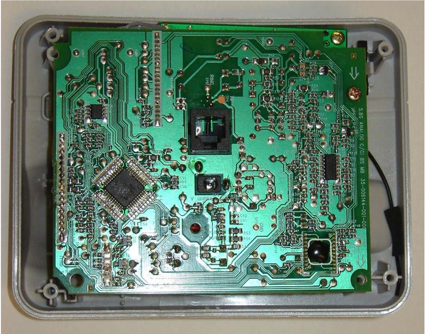
Vtech ia5823 Base PCB
