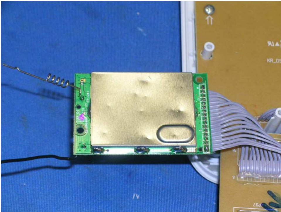
Base Unit Oscillator PCB comp side with shielding
