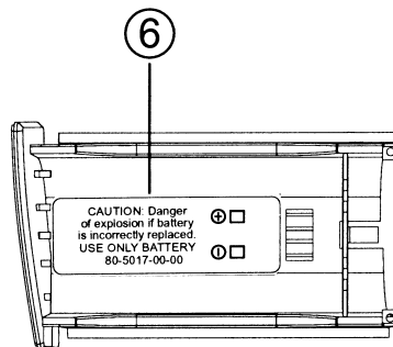
30-0940 battery drawer
