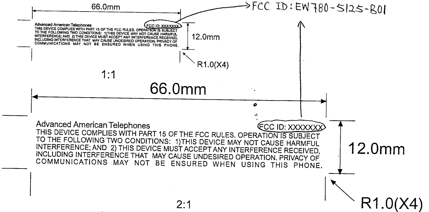
AT&T 1430 BASE BTMT- FCCID (PART15) Engrave (C)
