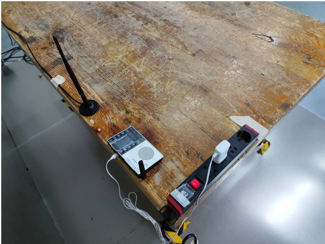
Conducted Emissions Side View-Adapter A318-050100W-US2
