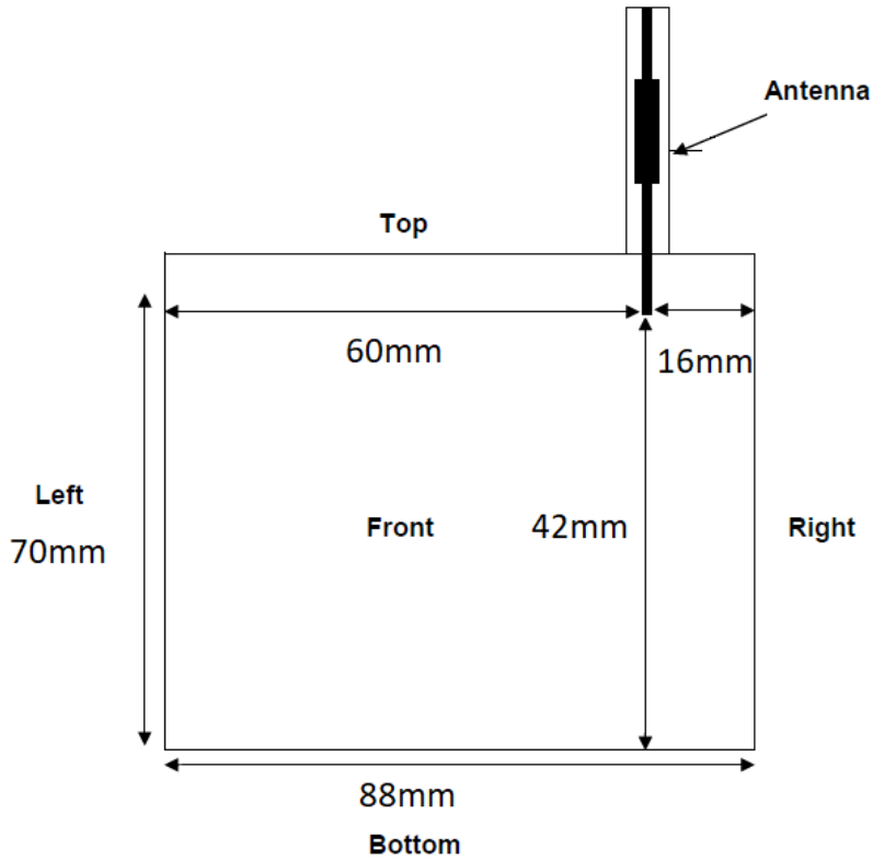
Antenna extended configuration
