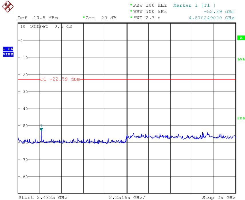
802.11g, Middle Channel, Plot B
