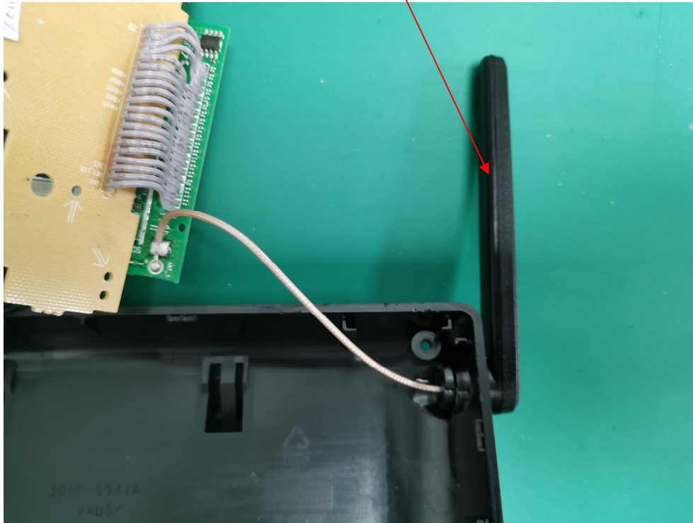
DECT Antenna 1
