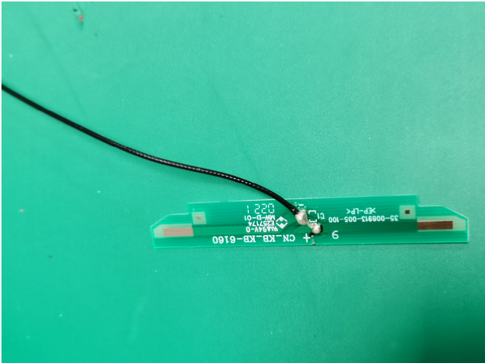
DECT Antenna 0
