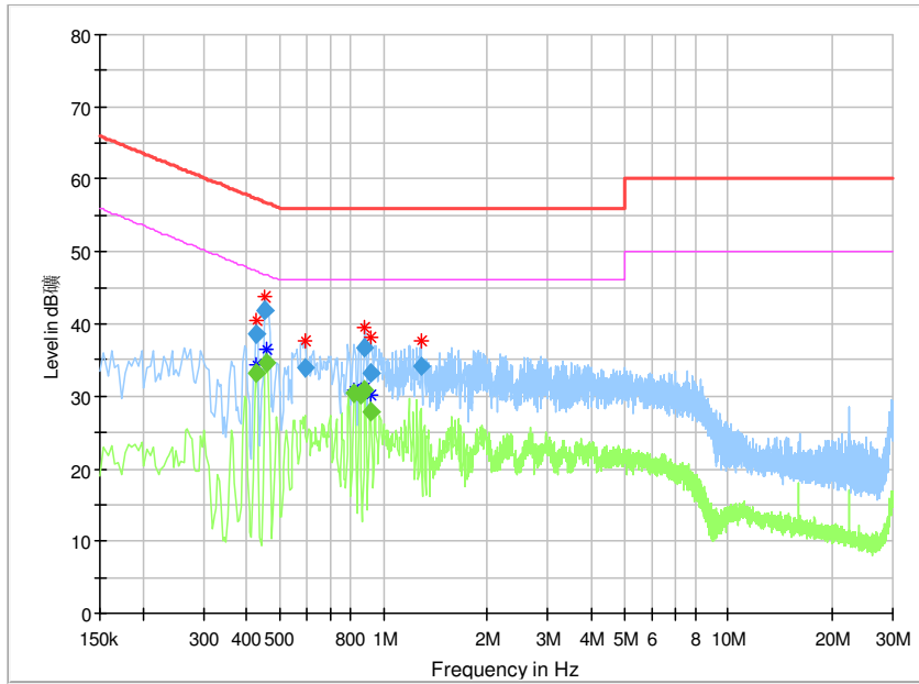
Full Spectrum
