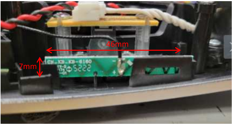
Antenna 2 Dimensions:
