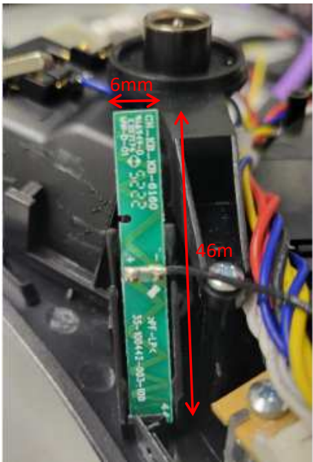
Antenna 2 Dimensions:
