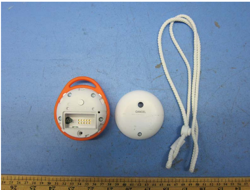
Figure 2 - Back View
